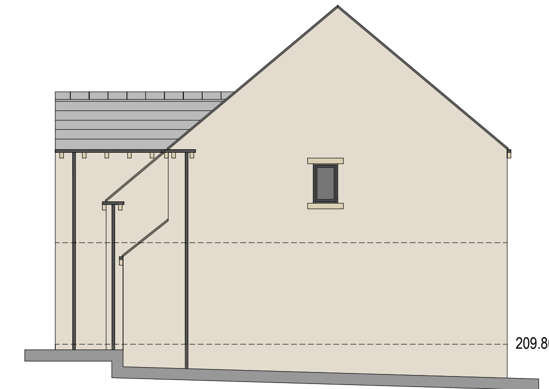
NORTH ELEVATION
