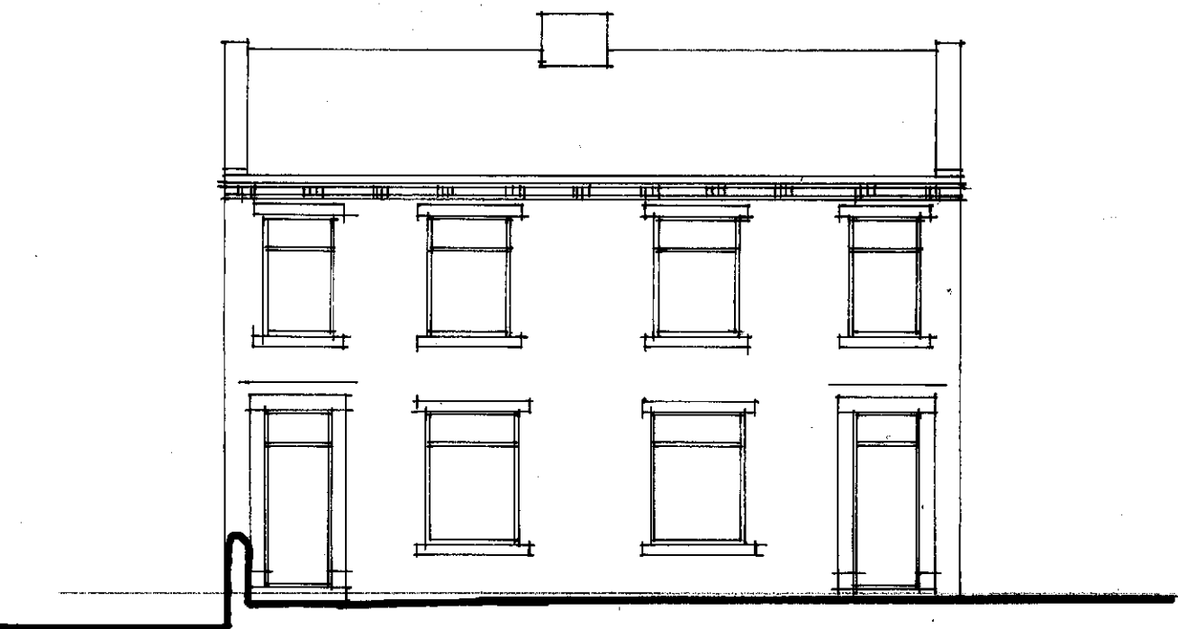
WEST 1:100
