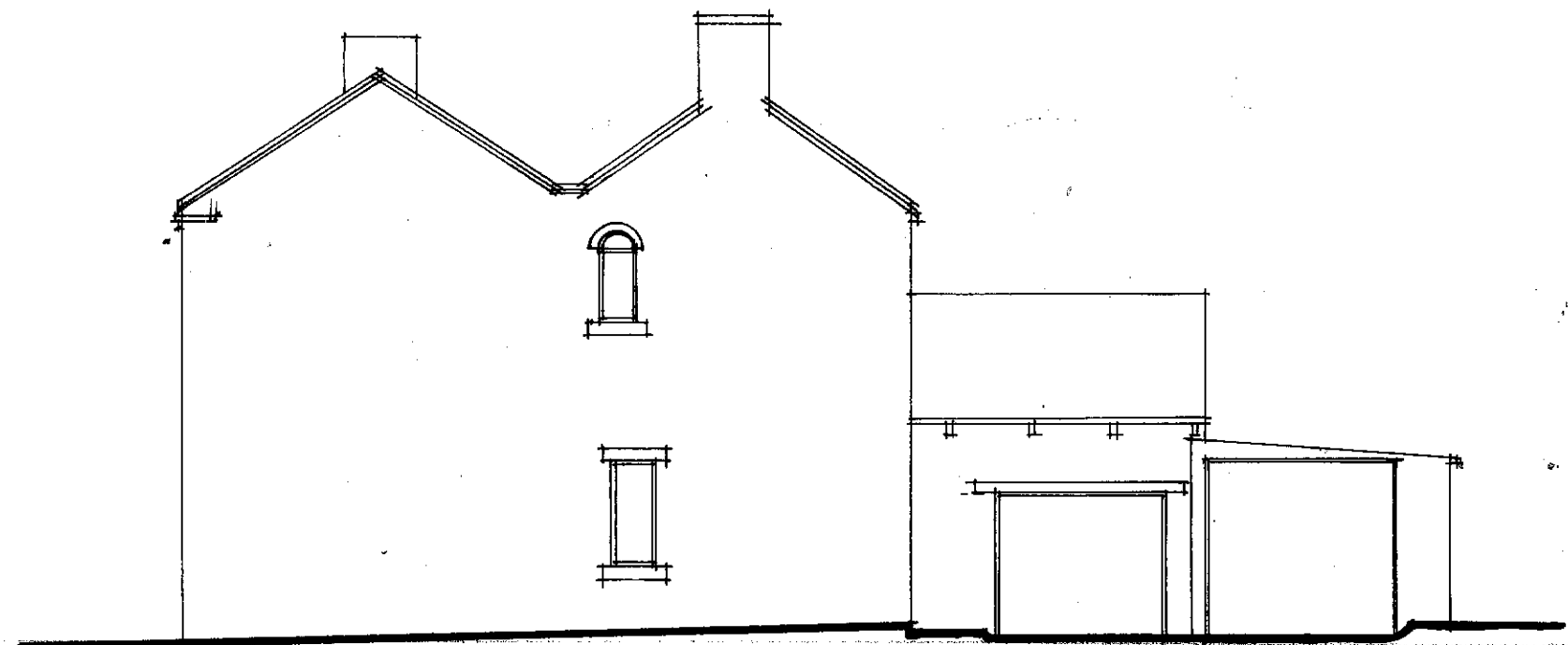
SOUTH 1:100
