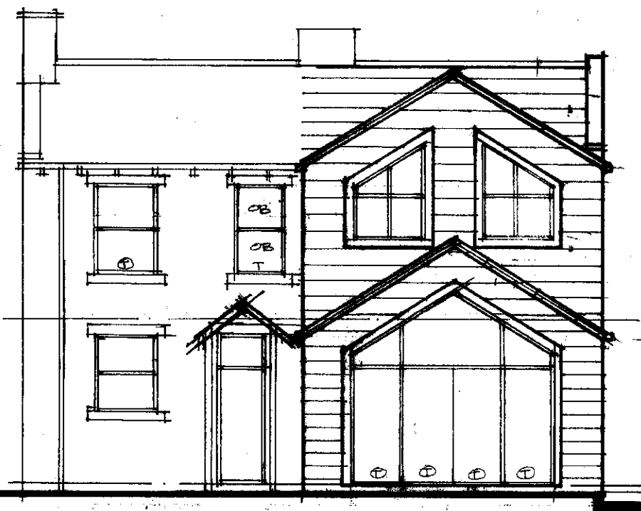
EAST 1:100
