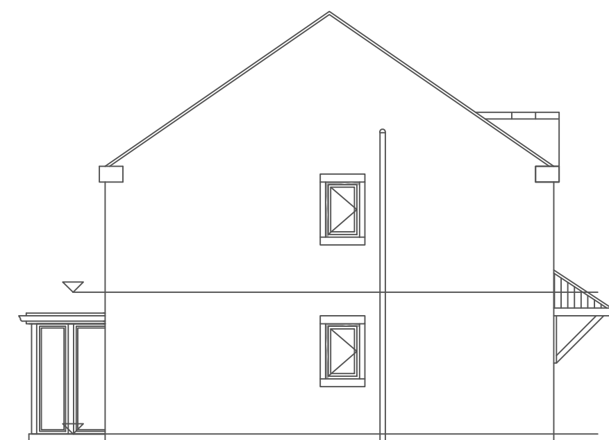
WEST ELEVATION (SIDE) 1:100
