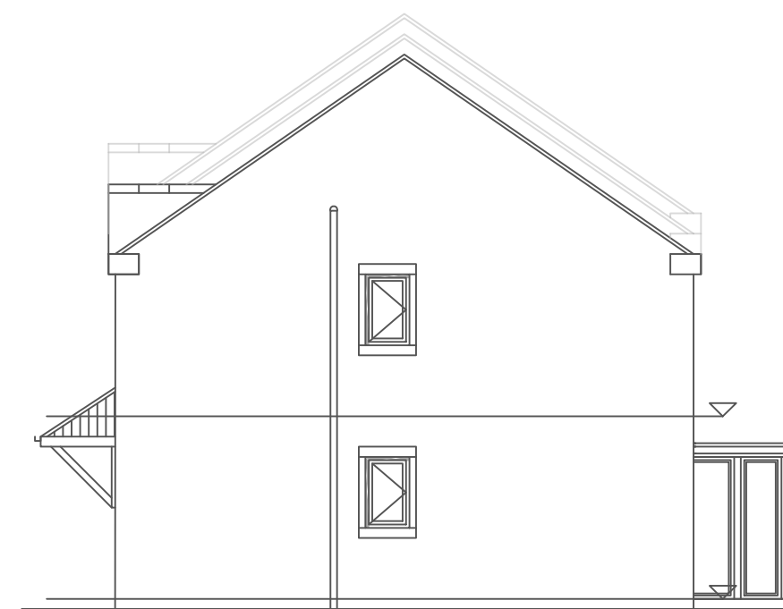
EAST ELEVATION (SIDE) 1:100
