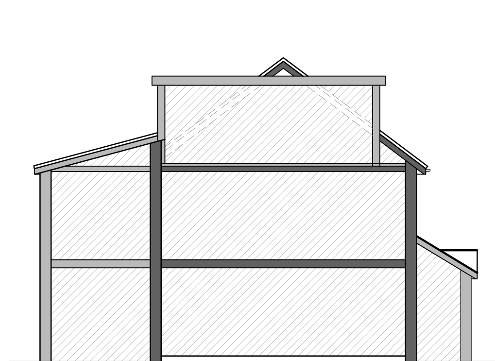
PROPOSED SECTION
