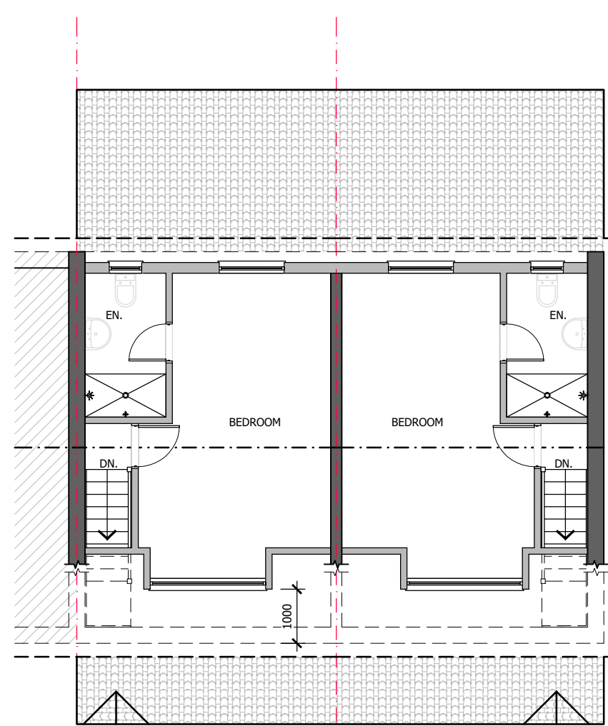
PROPOSED LOFT PLAN
