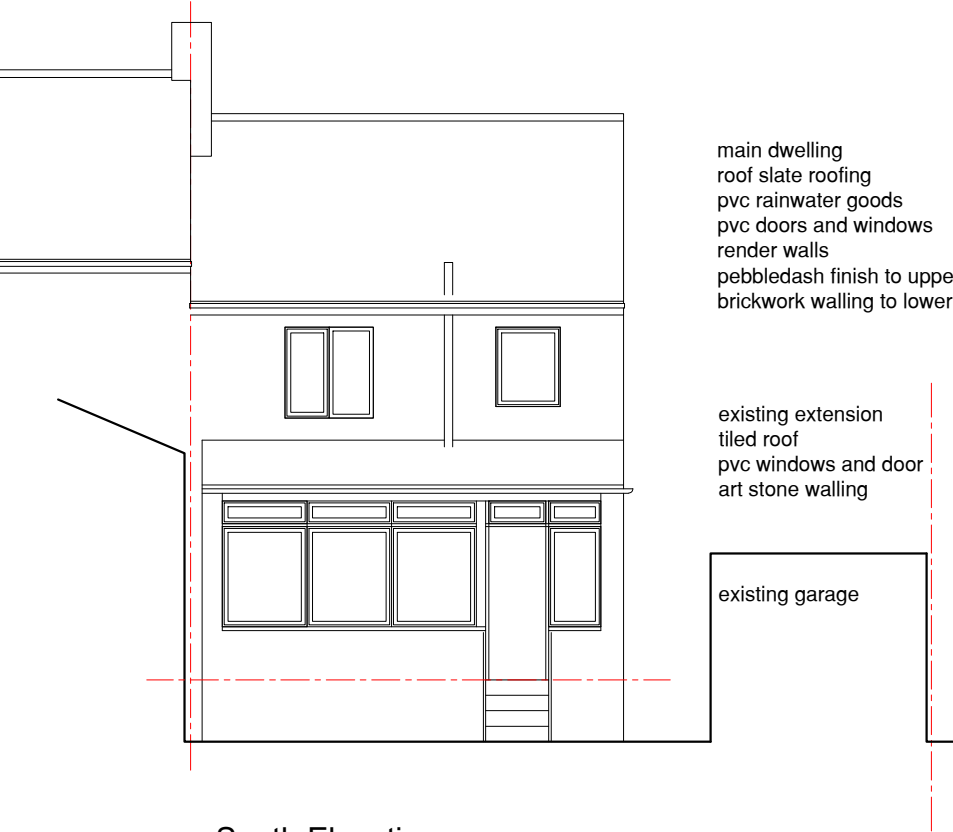
South Elevation
