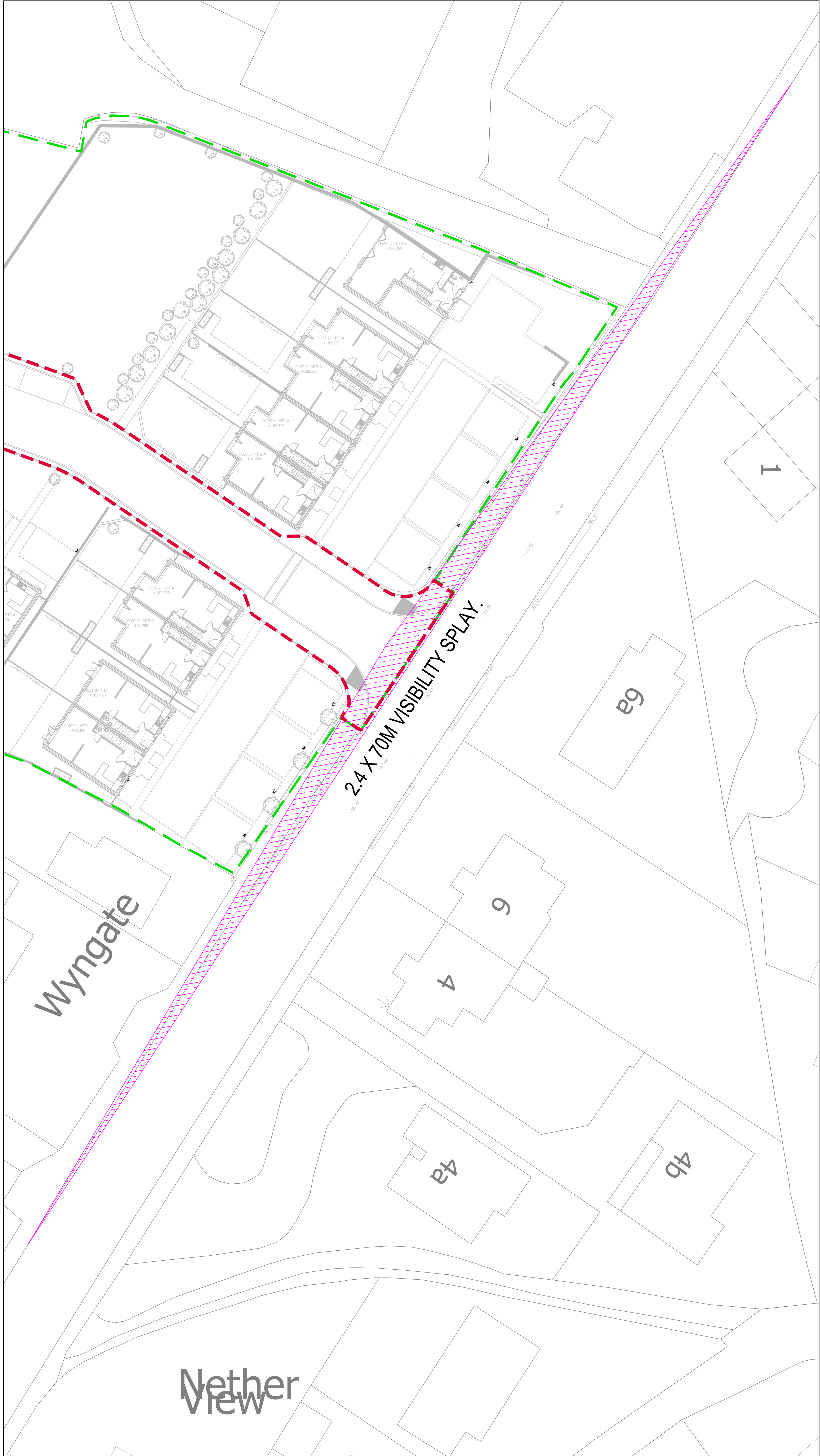
Site Entrance Visibility Splay (2.4m x 70m) (SCALE 1:250)
