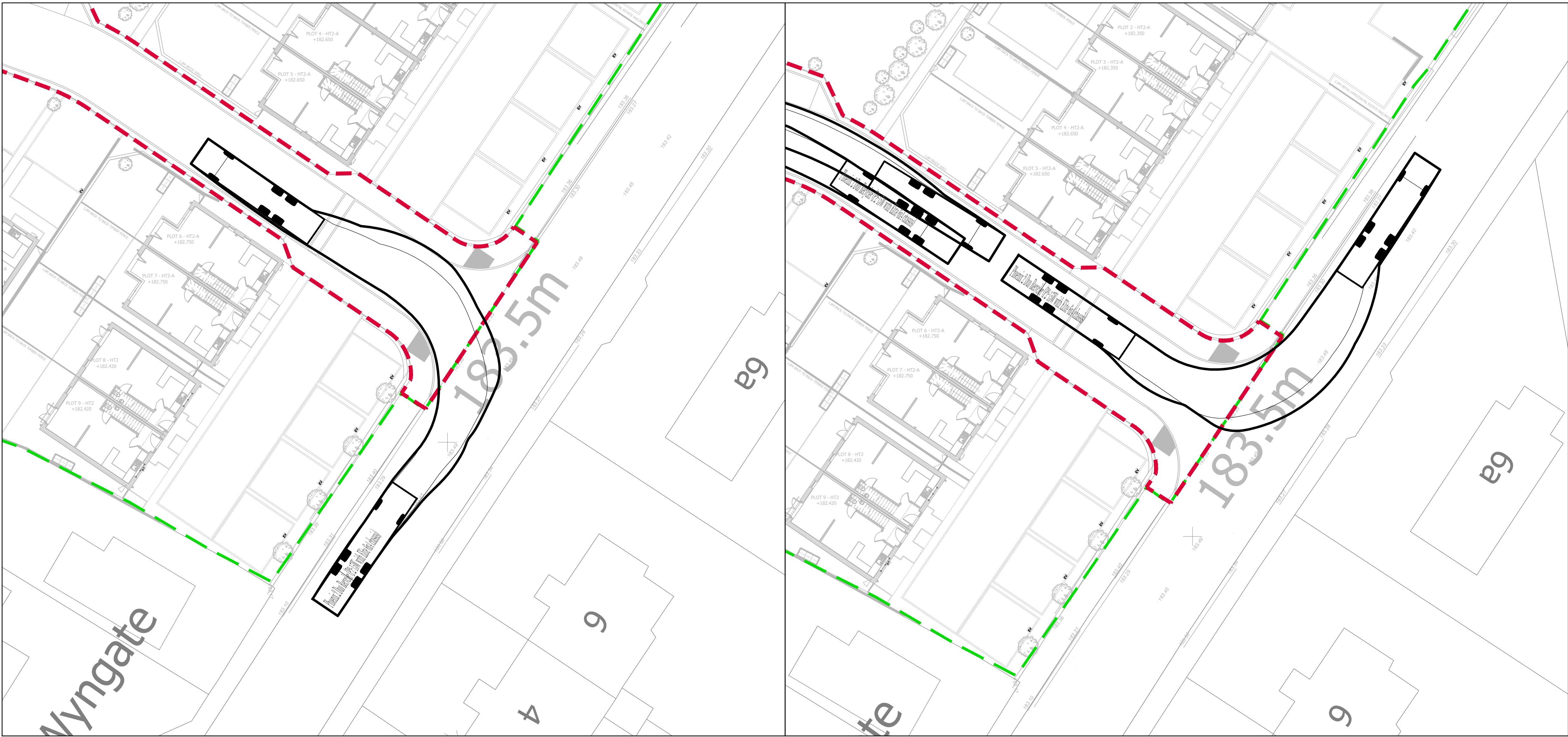
SITE ENTRANCE TRACKING DETAILS (SCALE 1:200)
