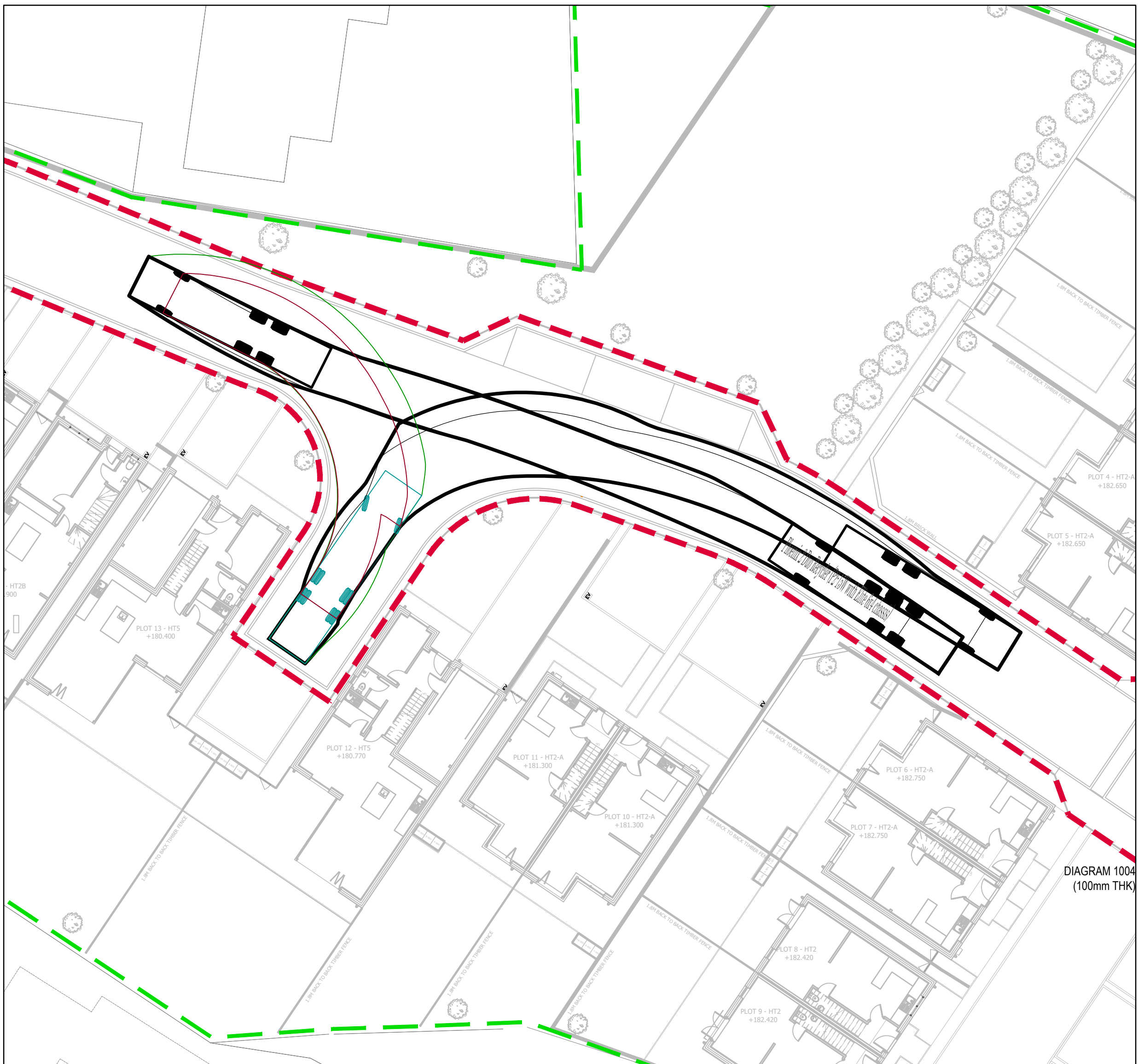
Turning Head Tracking Details (SCALE 1:200)
