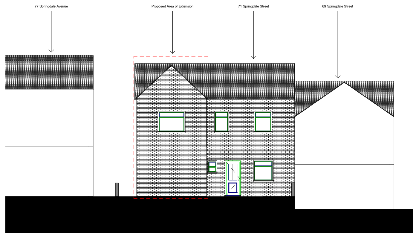
Proposed Back Elevation East Facing Elevation
