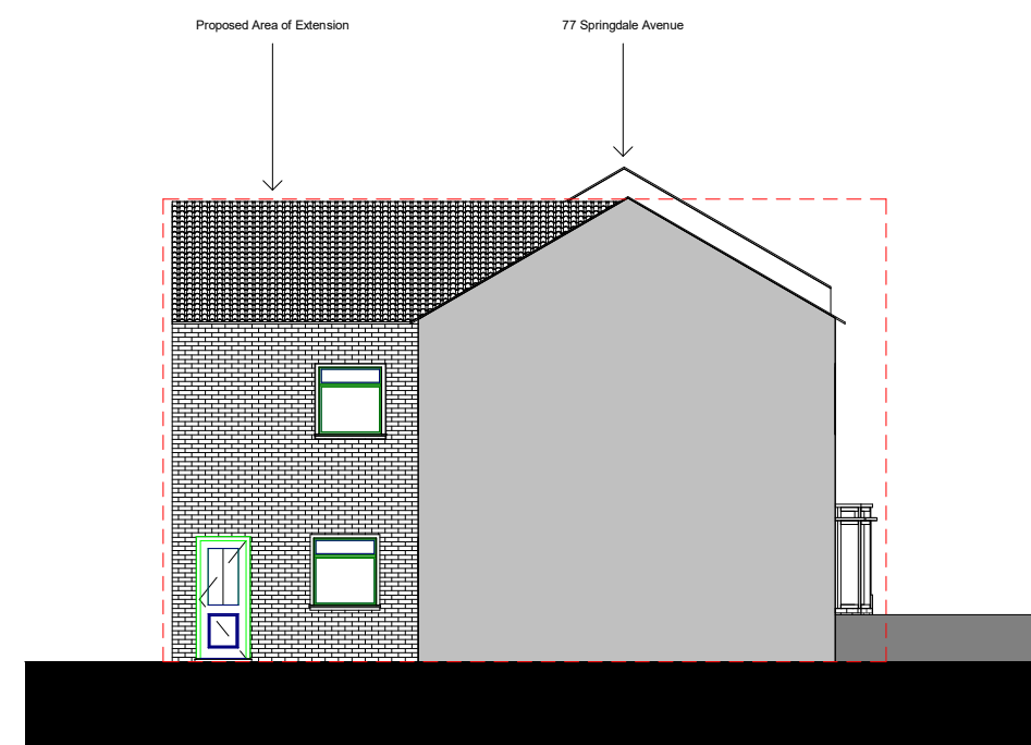
Proposed Side Elevation North Facing Elevation
