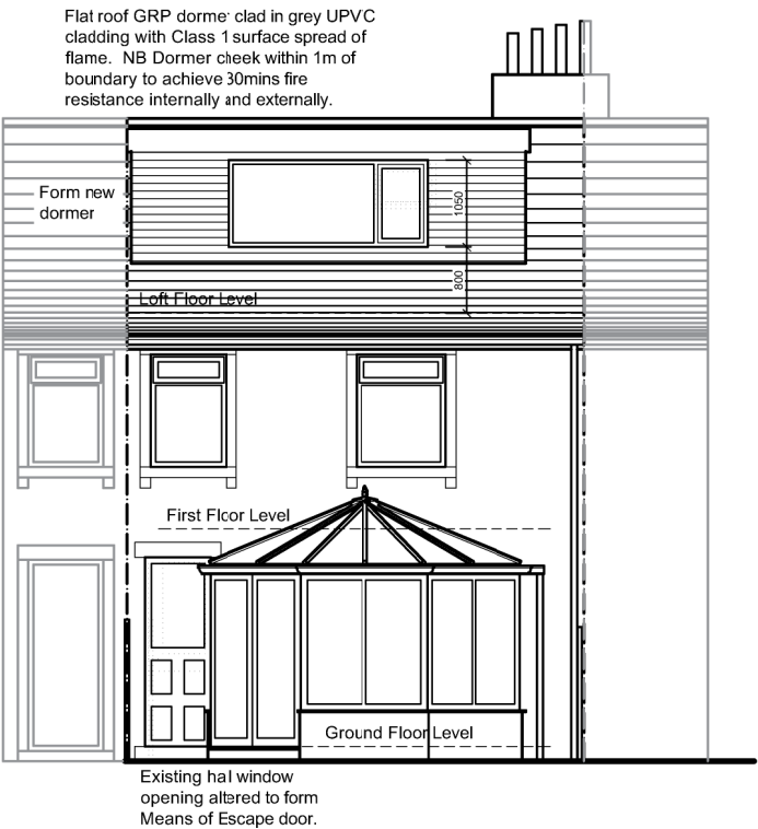
North (rear) Elevation
