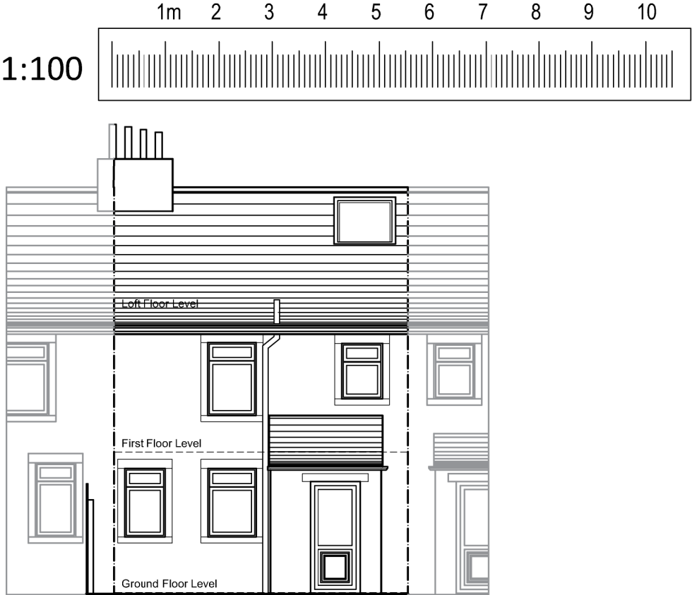
South (front) Elevation
