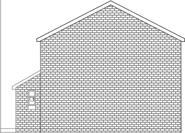
EXISTING SIDE ELEVATION (north west)
