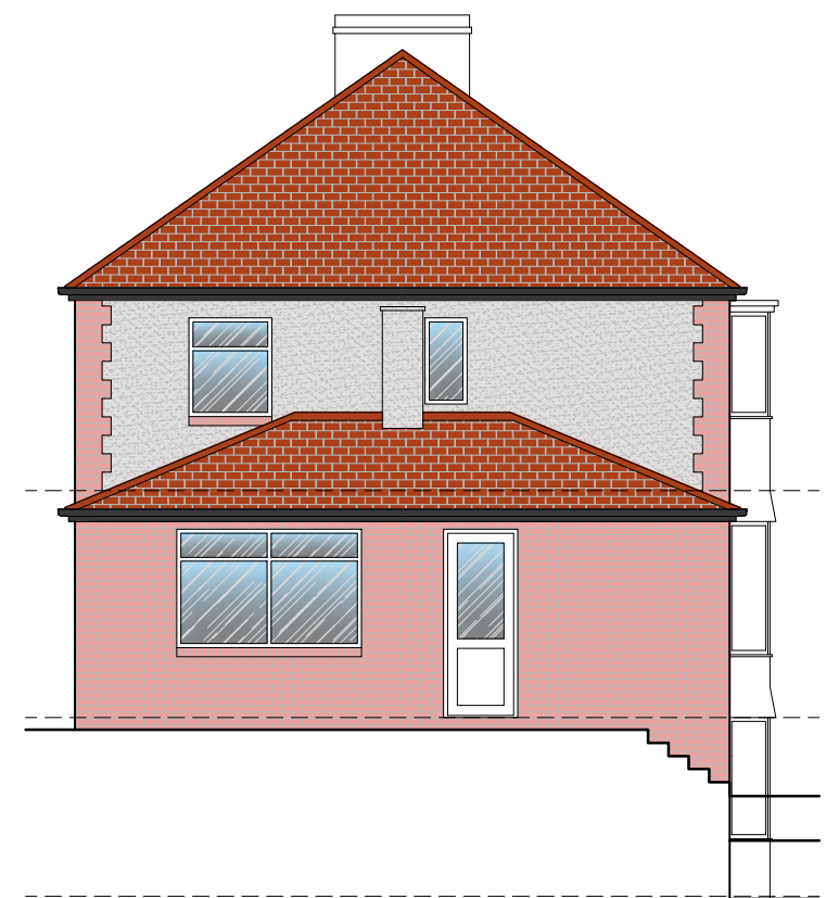
3. Existing West Elevation Scale 1:100
