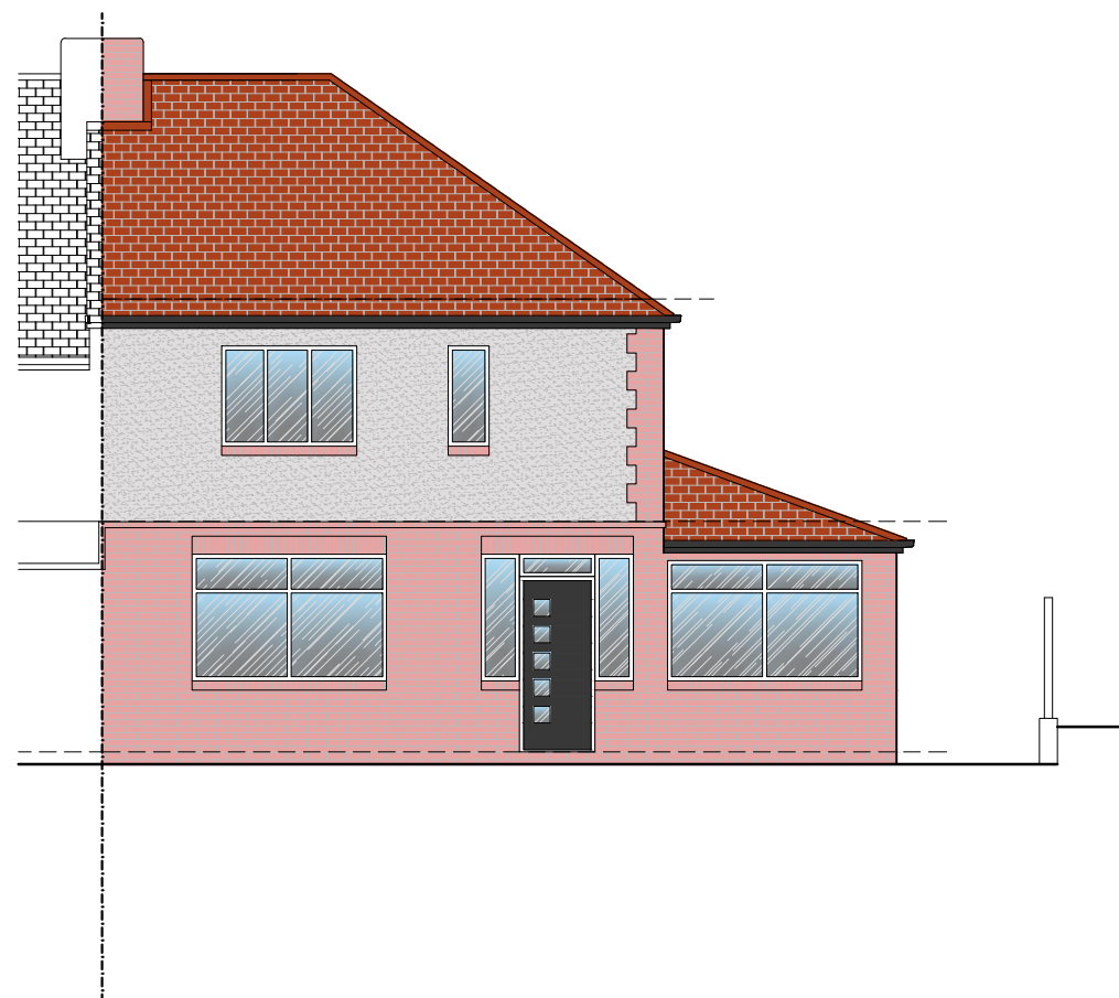
2. Existing North Elevation Scale 1:100
