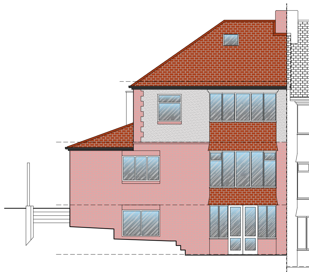
1. Existing South Elevation Scale 1:100
