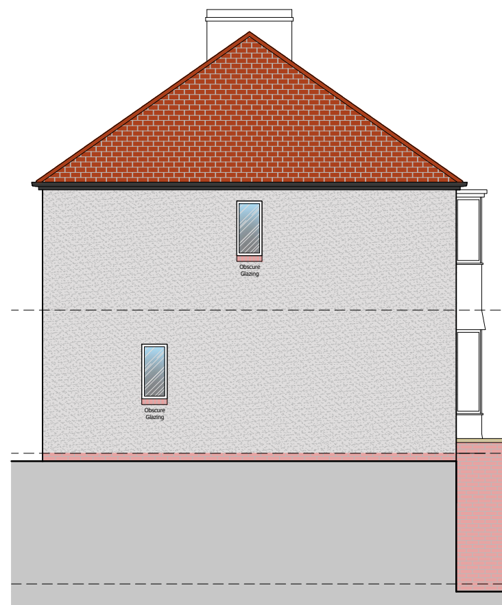
3. Proposed West Elevation Scale 1:100
