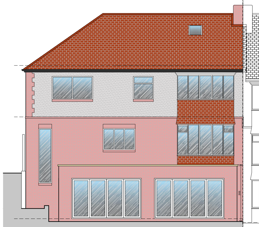
1. Proposed South Elevation Scale 1:100
