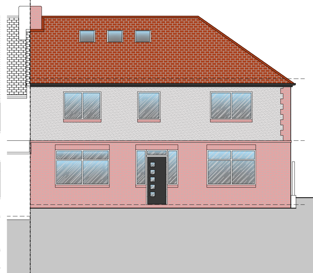
2. Proposed North Elevation Scale 1:100
