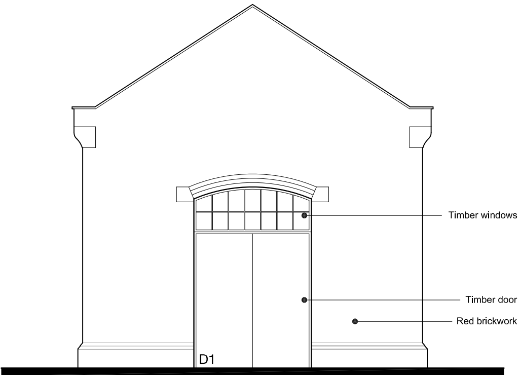
North Elevation
