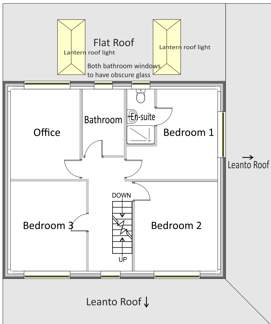
Proposed First Floor Plan Scale 1:100 (Ref: HD45DB47v3)
