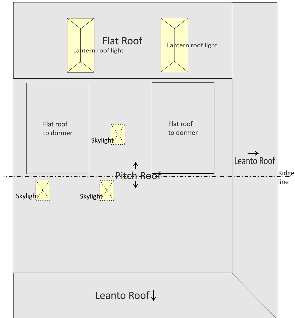
Proposed Roof Plan Scale 1:100 (Ref: HD45DB47v3)
