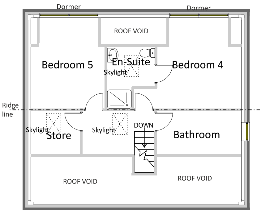
Proposed Second Floor Plan Scale 1:100 (Ref: HD45DB47v3)
