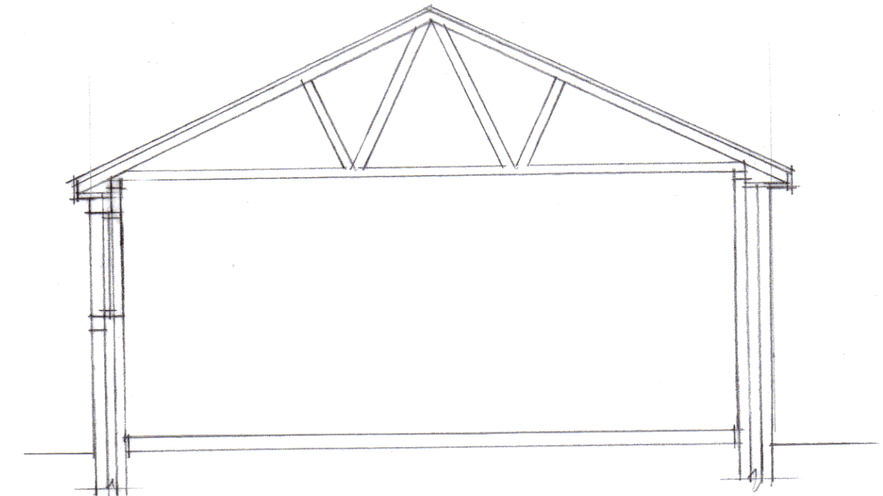
section
