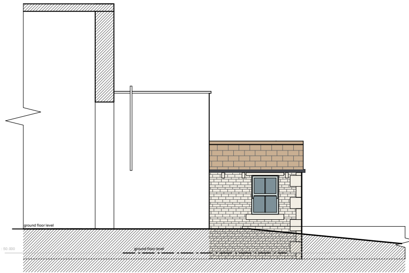
sectional elevation a-a - north west
