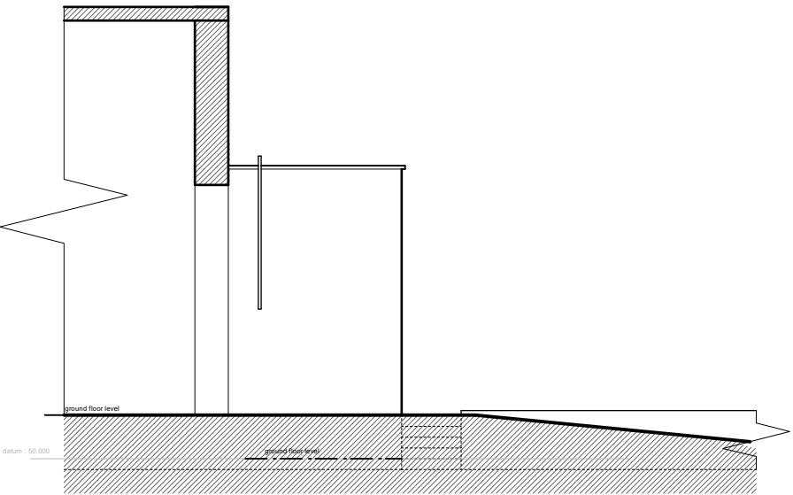
sectional elevation a-a - north west
