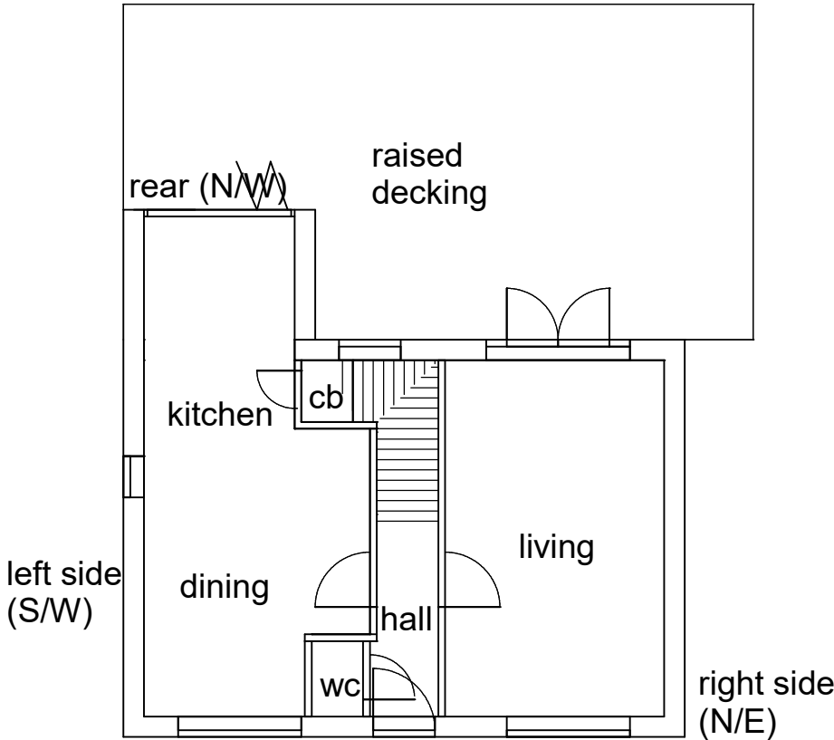
front (S/E) GROUND FLOOR LAYOUT
