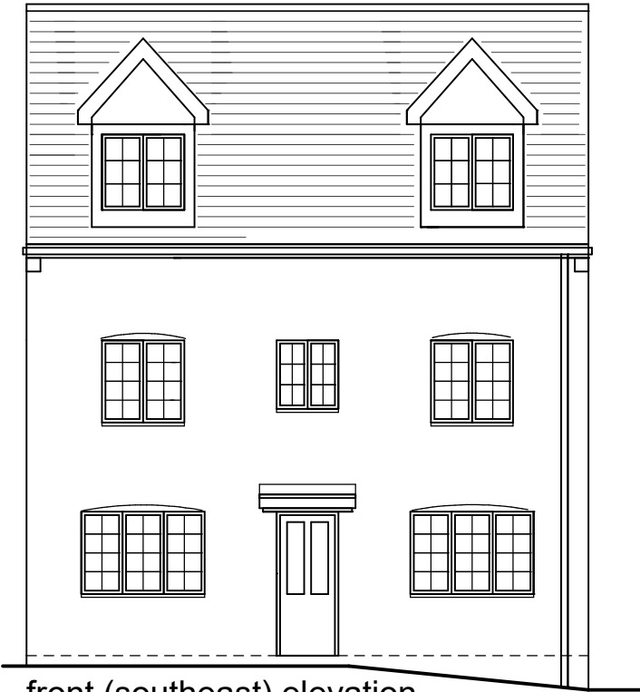
front (southeast) elevation
