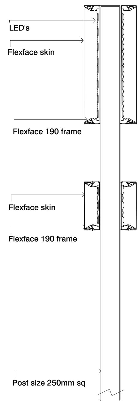
SECTION THROUGH - SCALE 1:20
