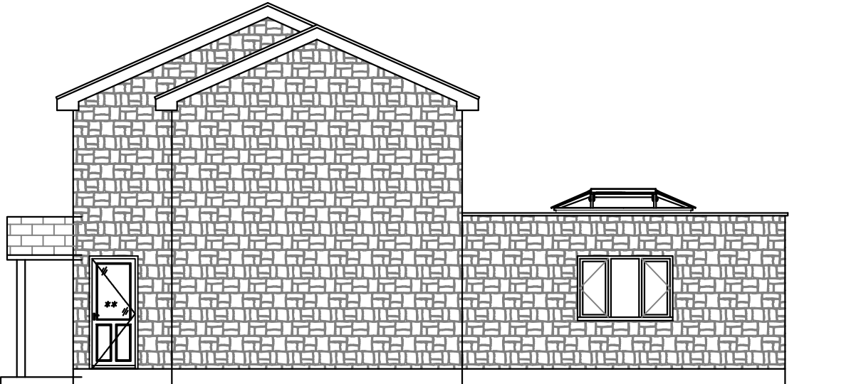
Side Elevation
