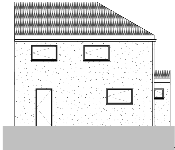
Proposed East South East (Front) 1 : 100
