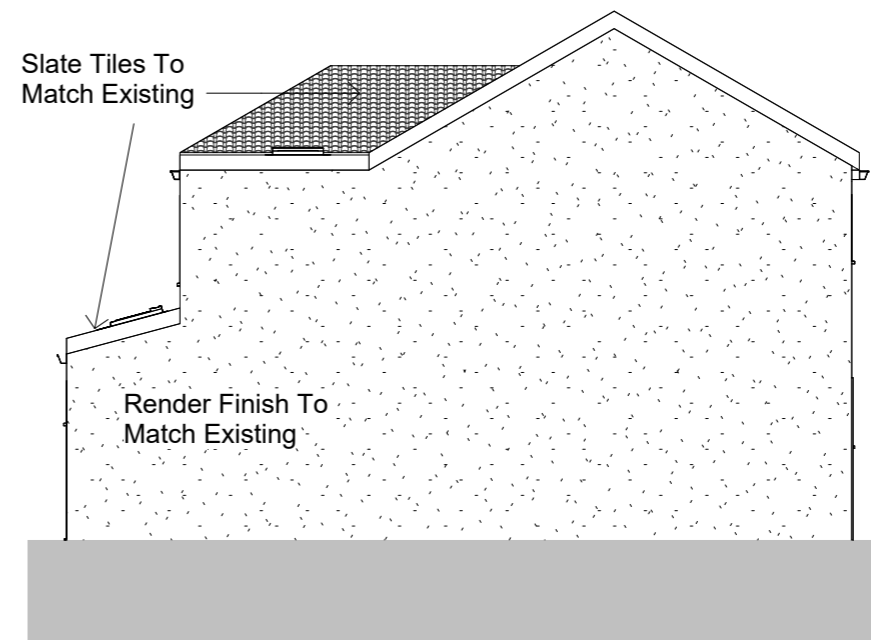
Proposed South West South (Left) 1 : 100
