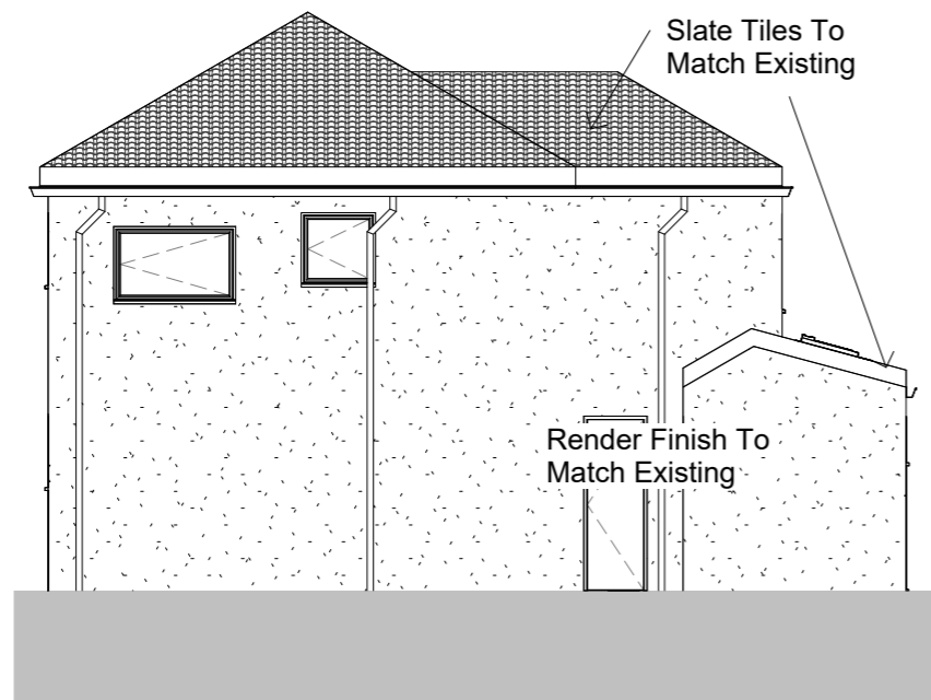
Proposed North East North (Right) 1 : 100
