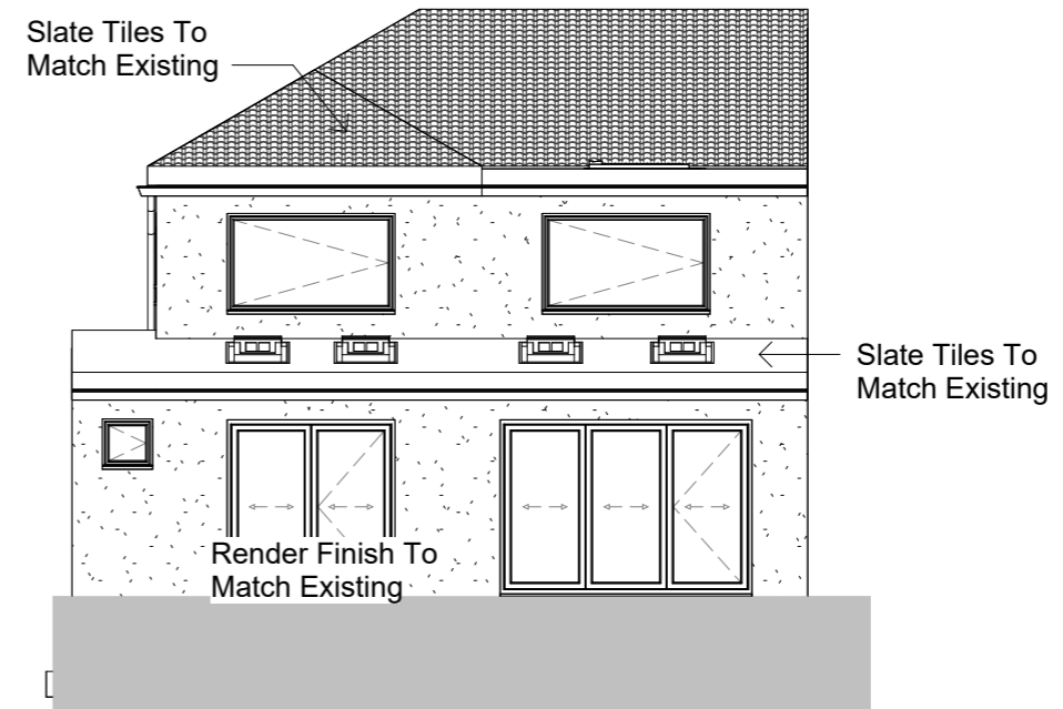
Proposed West North West (Rear) 1 : 100
