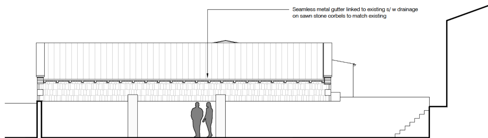
Western Elevation 1: 100
