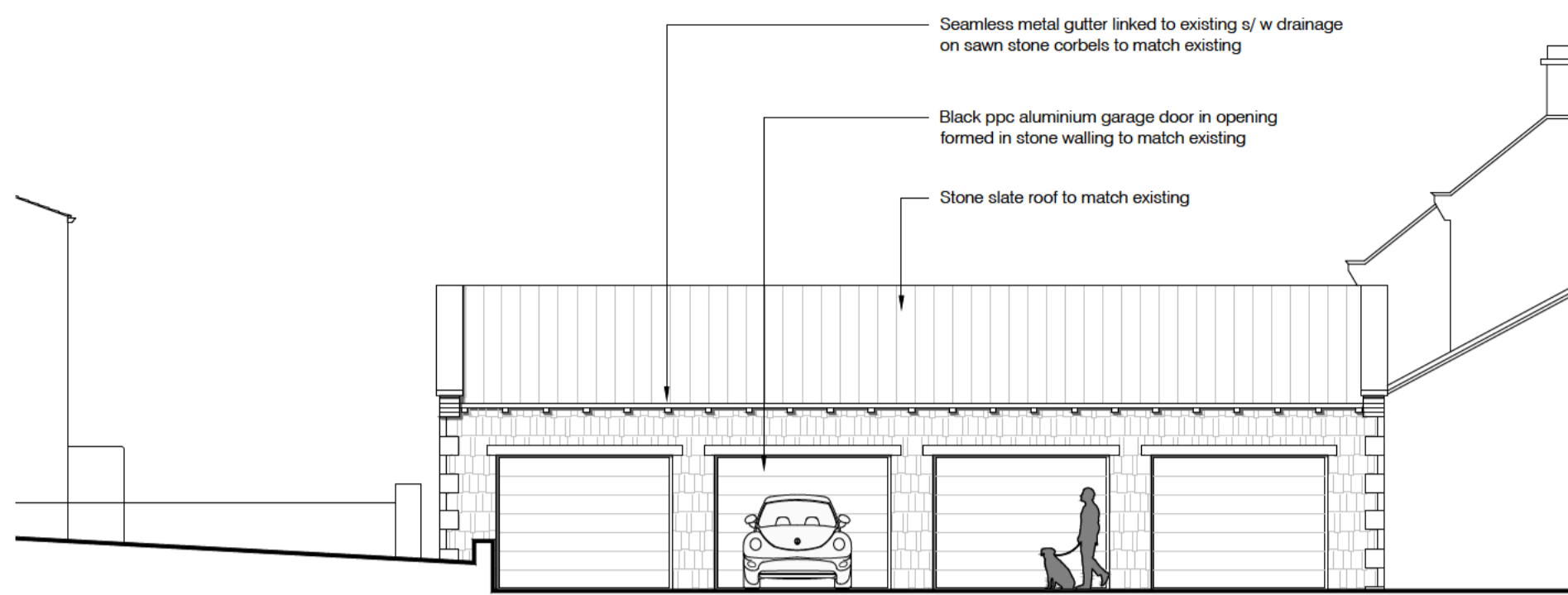
Eastern Elevation 1: 100
