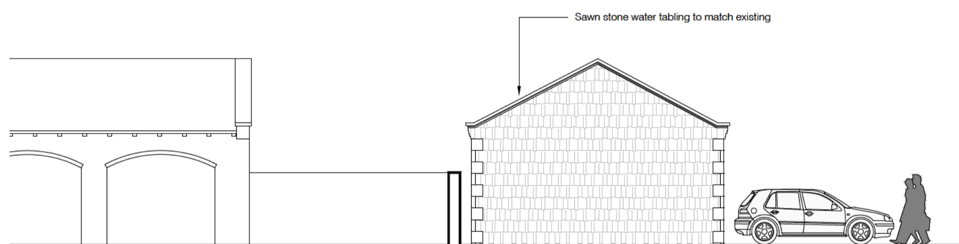
Southern Elevation 1: 100
