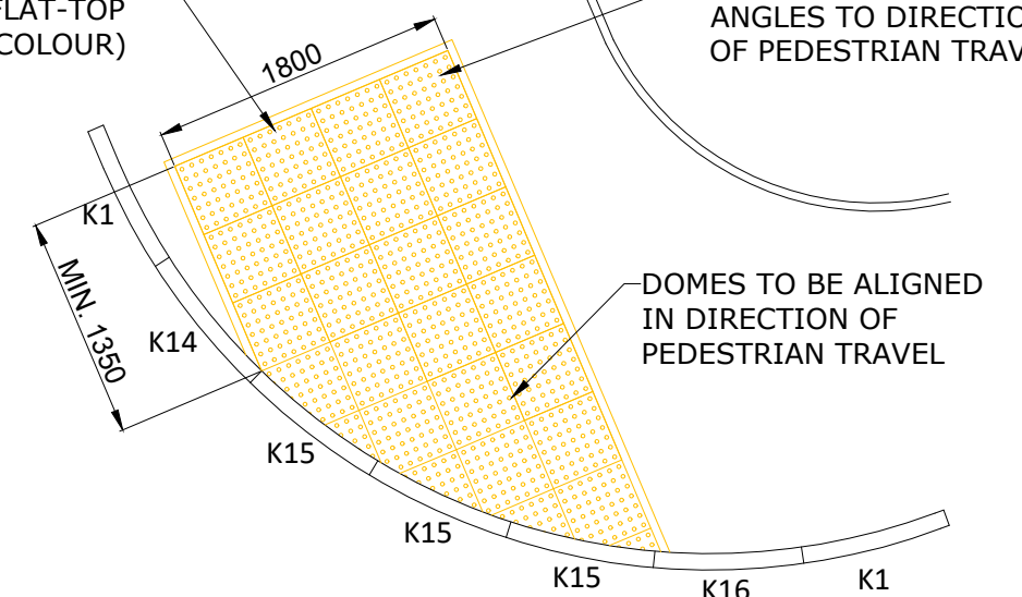
DETAIL C
