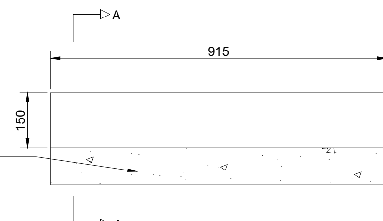
EDGING TYPE 1
