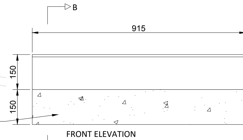
KERB TYPE 15
