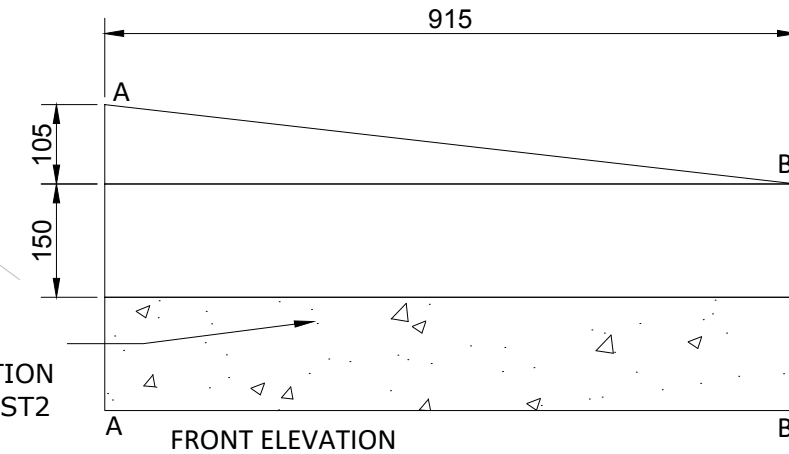
KERB TYPE 14
