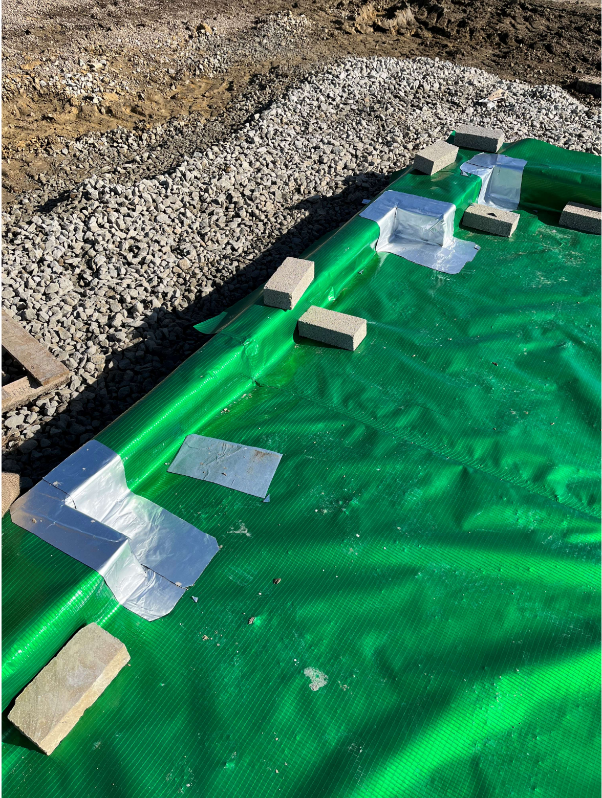
Plot 8 – Membrane layout with jointing
