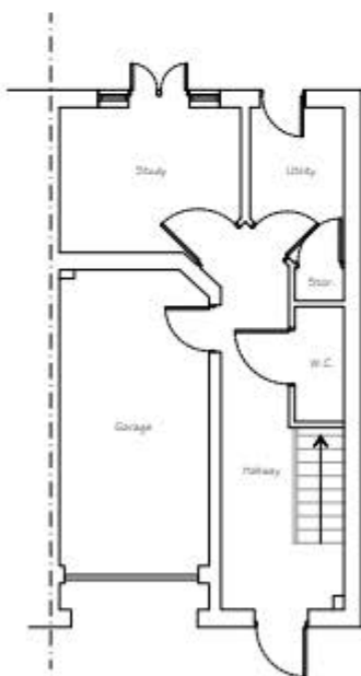
Ground Floor Plan As Existing
