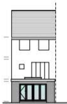
Rear Elevation As Proposed
