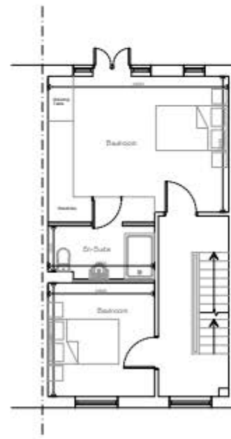
First Floor Plan As Proposed
