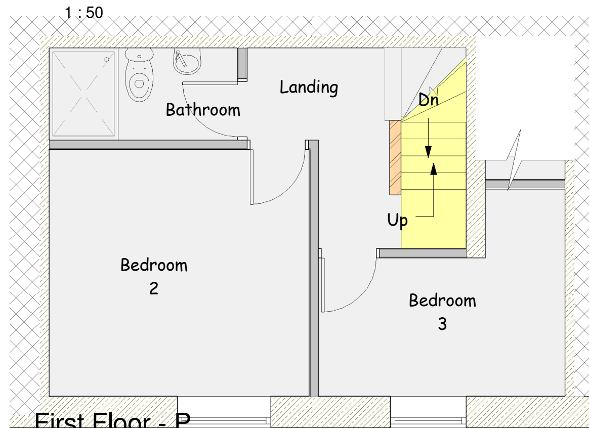
First Floor - P 1 : 50
