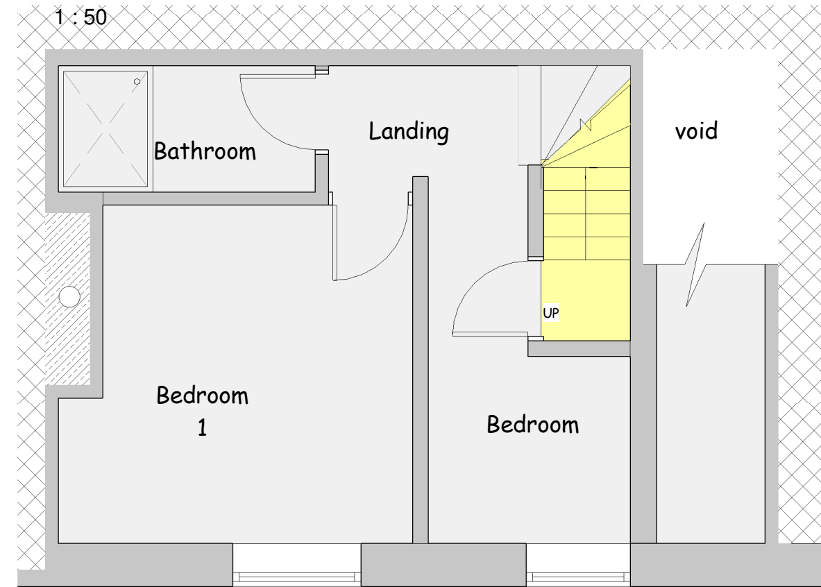
First Floor 1 : 50
