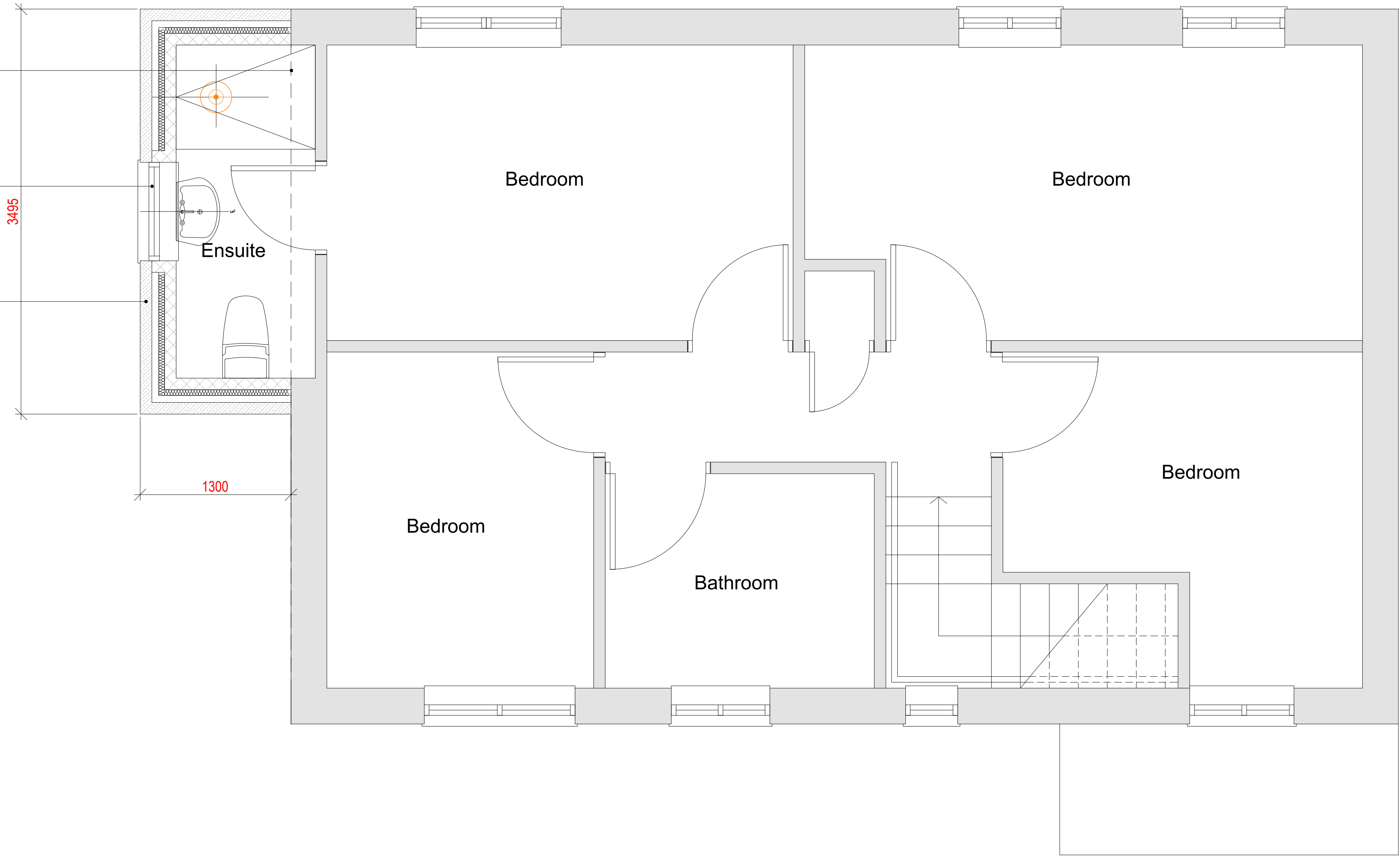
PROPOSED FIRST FLOOR PLAN 1:25
