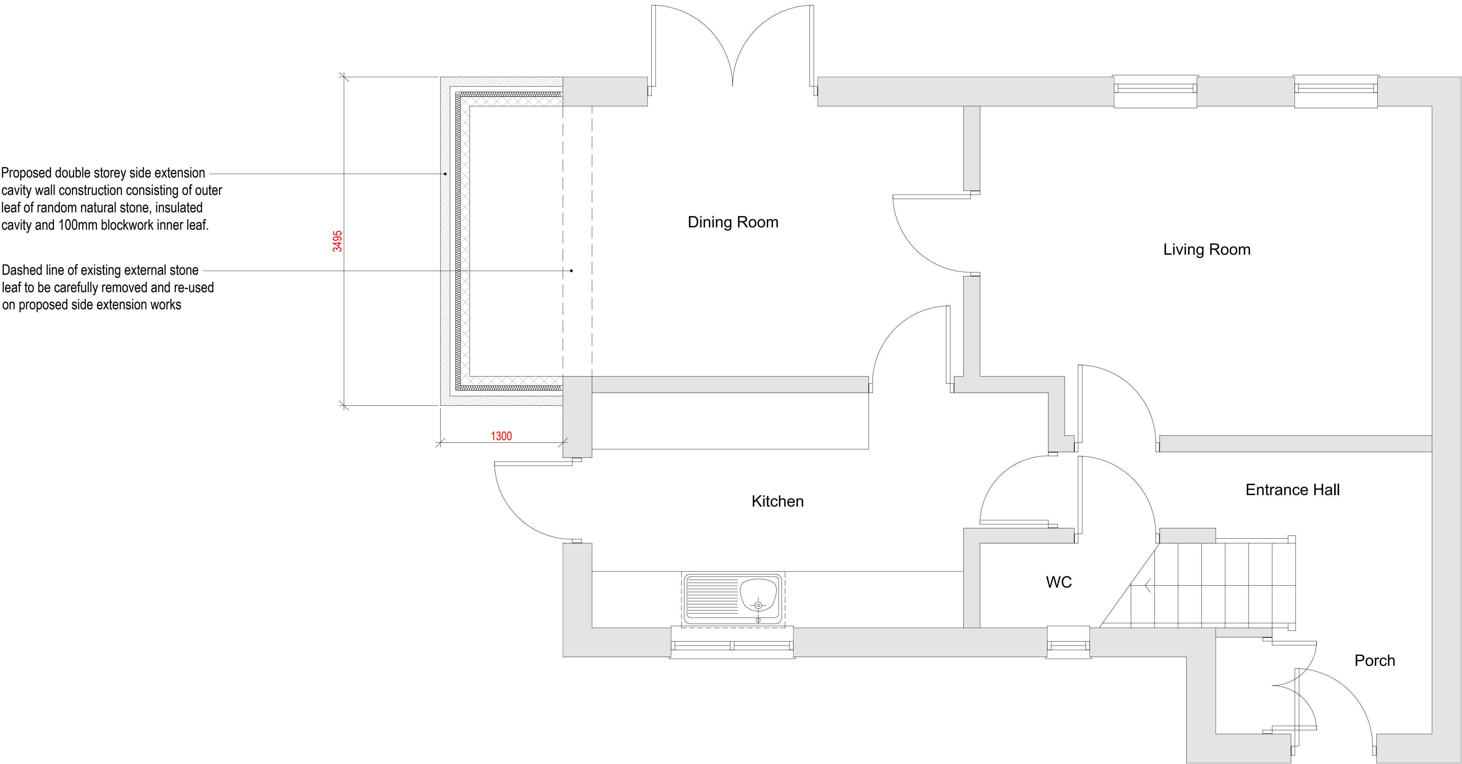
PROPOSED GROUND FLOOR PLAN 1:25
