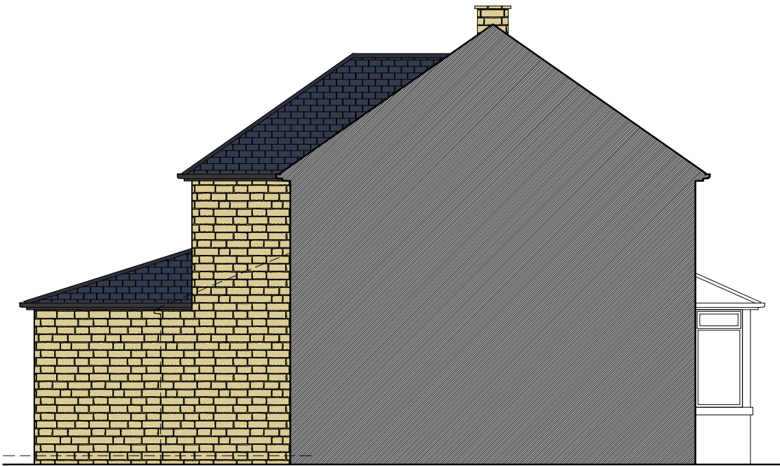
4. Proposed West Elevation Scale 1:100
