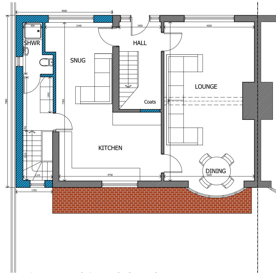
2. Proposed Ground Floor Plan Scale 1:100
