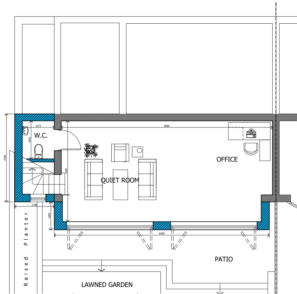
1. Proposed Basement Plan Scale 1:100
