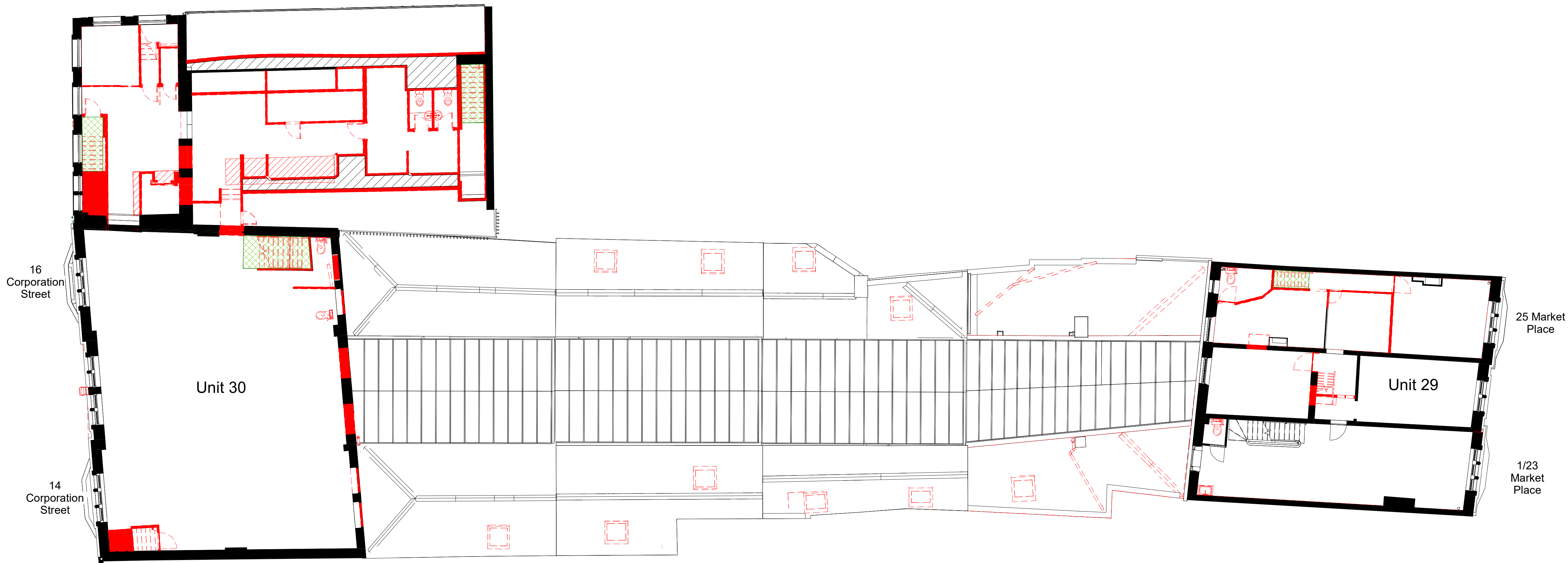
1 Second Floor Removals Plan 1 : 100
