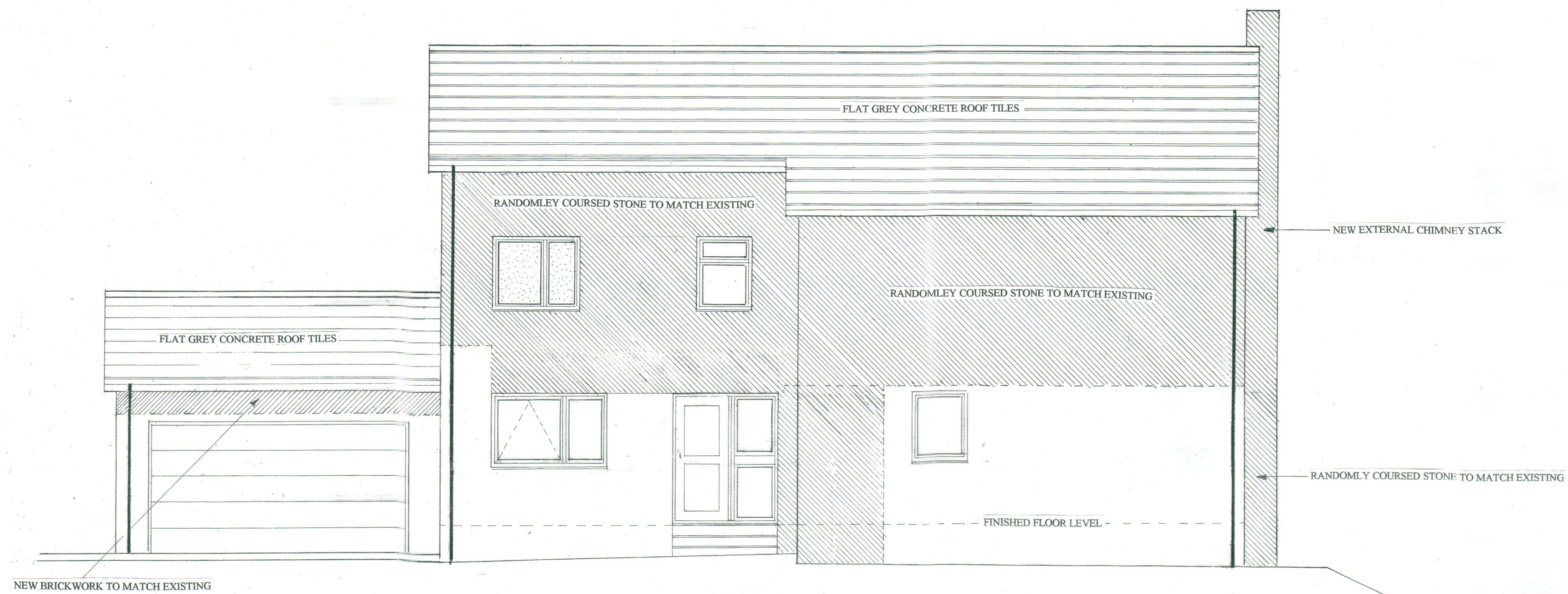
PROPOSED SOUTH WEST ELEVATION SCALE 1:50
