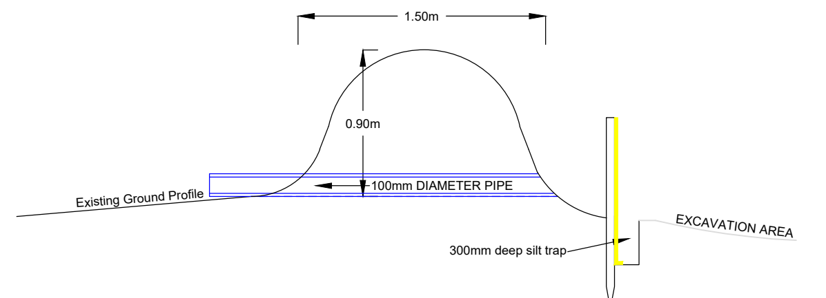
SECTION B-B THRO' PROPOSED BUND INC STRAW BALES Scale 1:25
