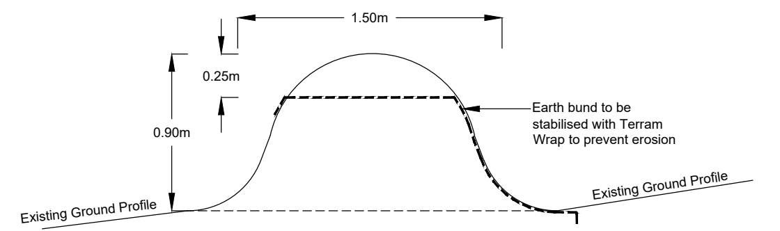
SECTION A-A THRO' PROPOSED BUND Scale 1:25
