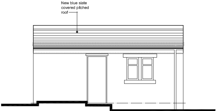
WEST ELEVATION (side)
