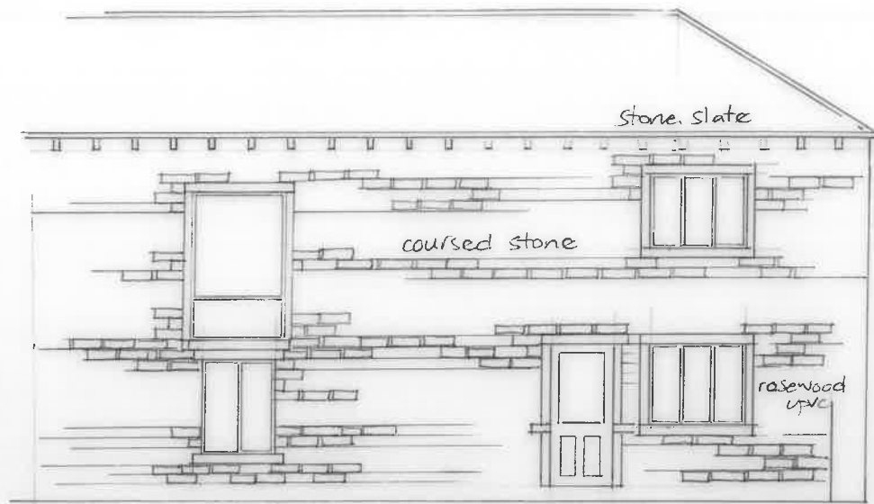
Elevations - Existing
