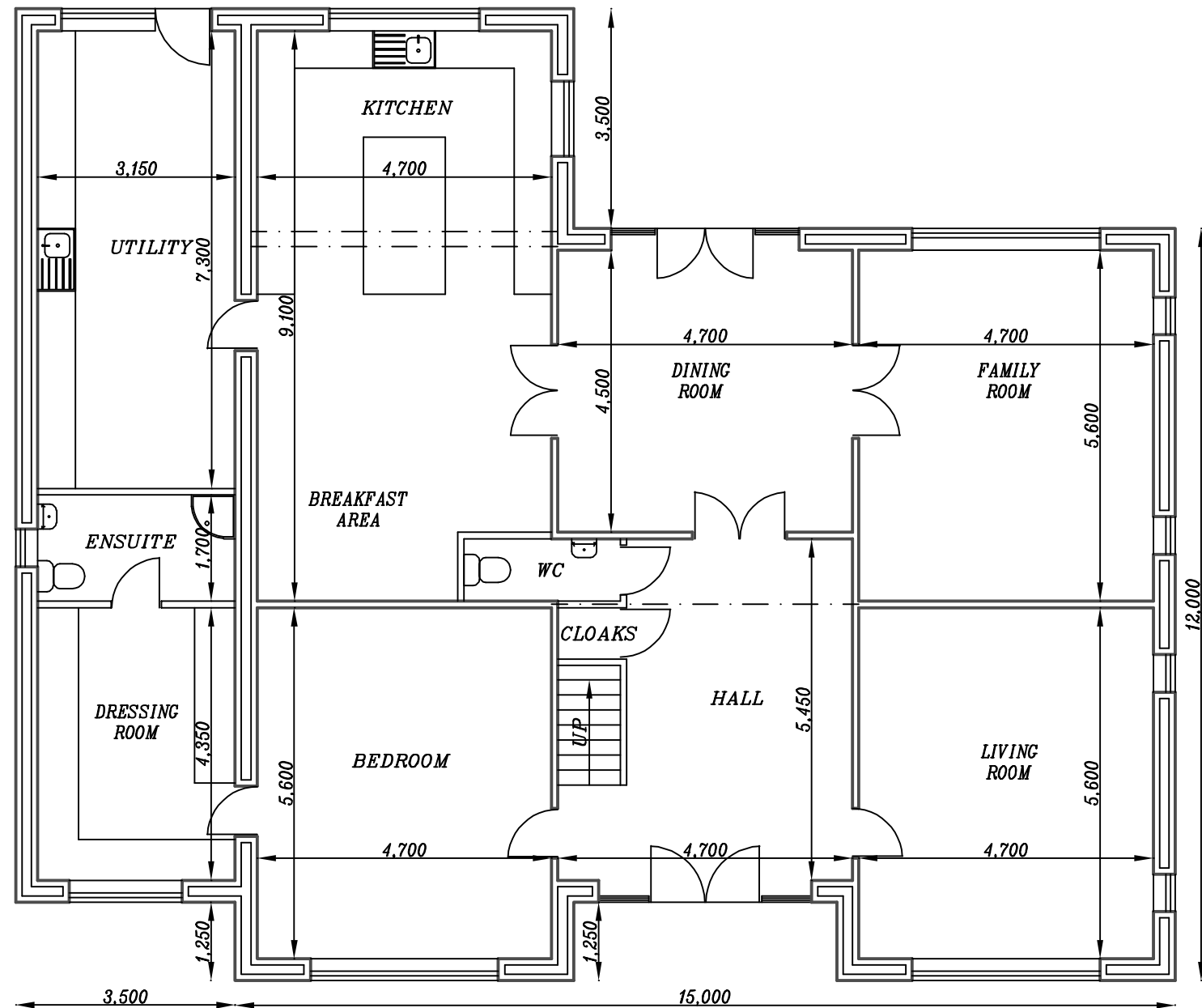
PROPOSED GROUND FLOOR PLAN (24 PROSPECT TERR)
