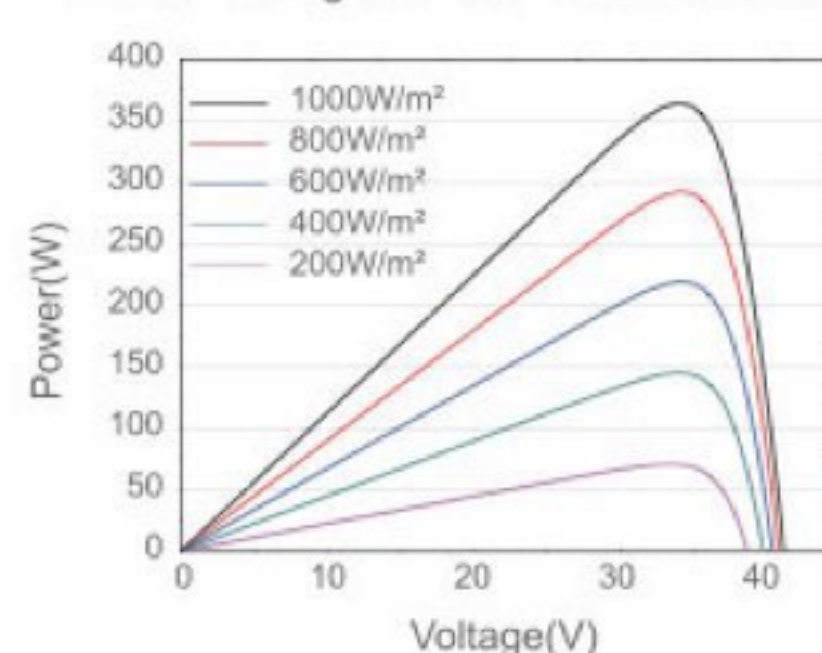
Power-Voltage Curve JAM60S21-365/MR
