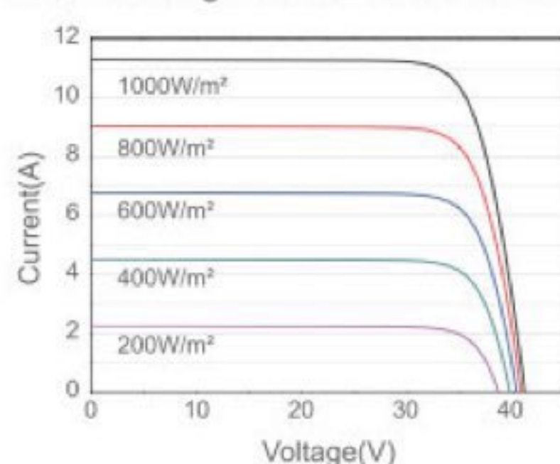
Current-Voltage Curve JAM60S21-365/MR
