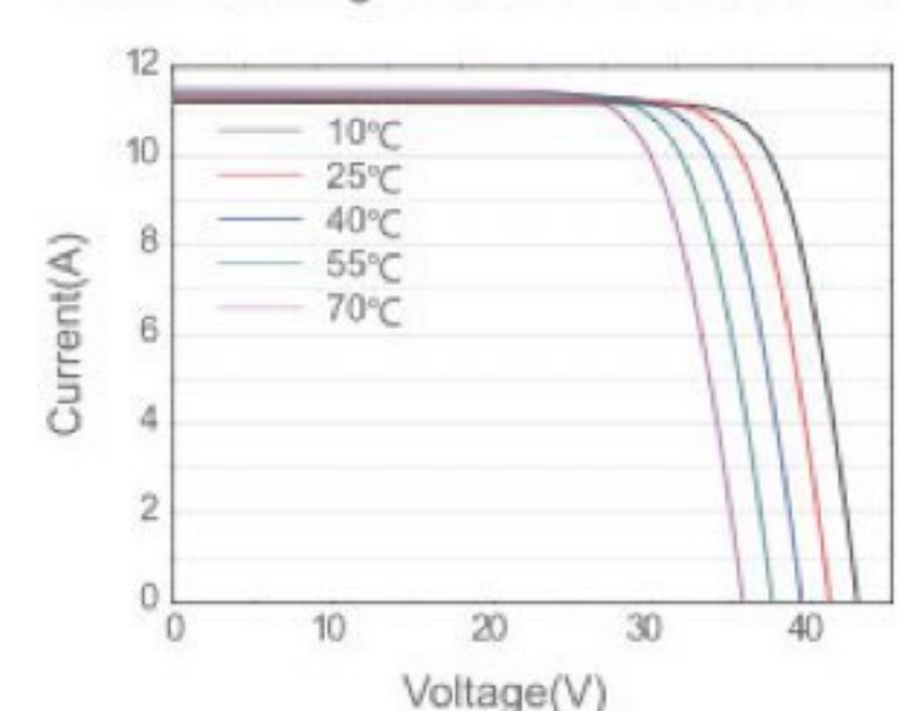
Current-Voltage Curve JAM60S21-365/MR
