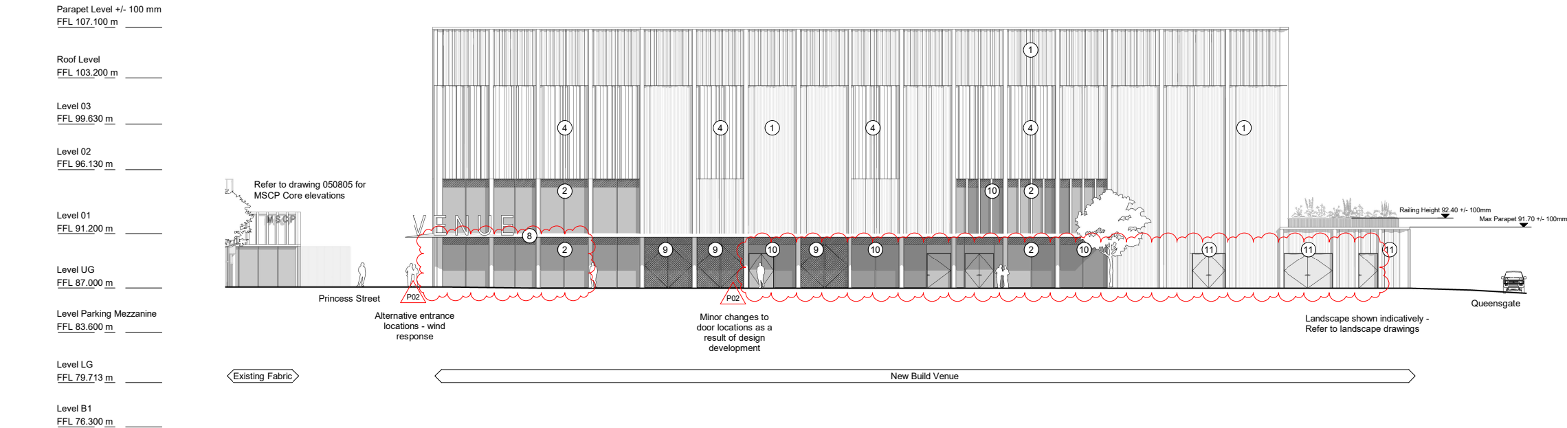
1 Proposed Elevation West 1 : 200
