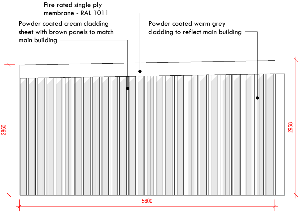
Bin Store Old Leeds Road Elevation 1 : 50
