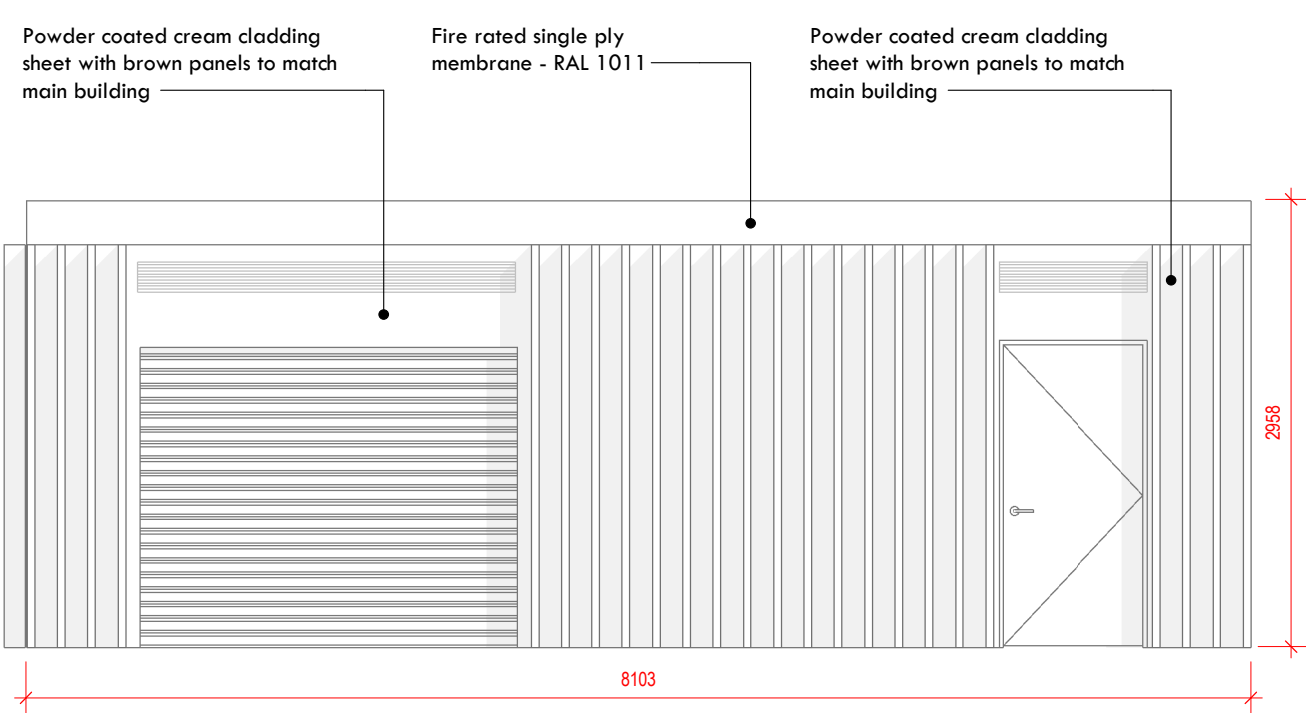
Bin Store Front Elevation 1 : 50
