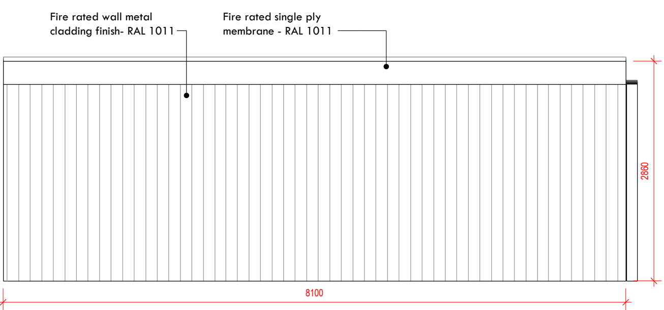
Bin Store Rear Elevation 1 : 50
