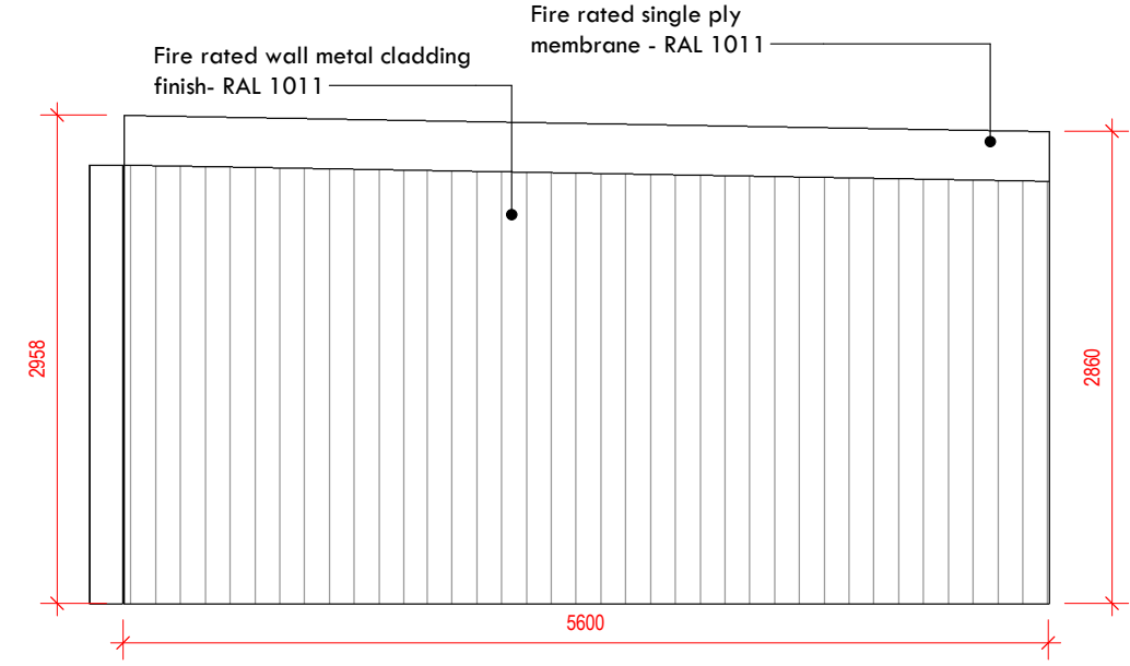
Bin Store Side Elevation 1 : 50
