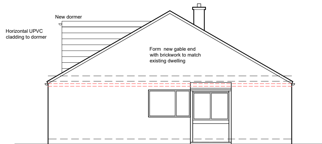
Side Elevation
