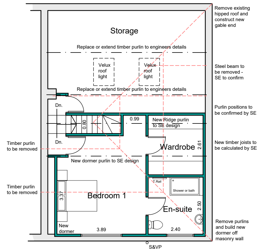
Roof Plan
