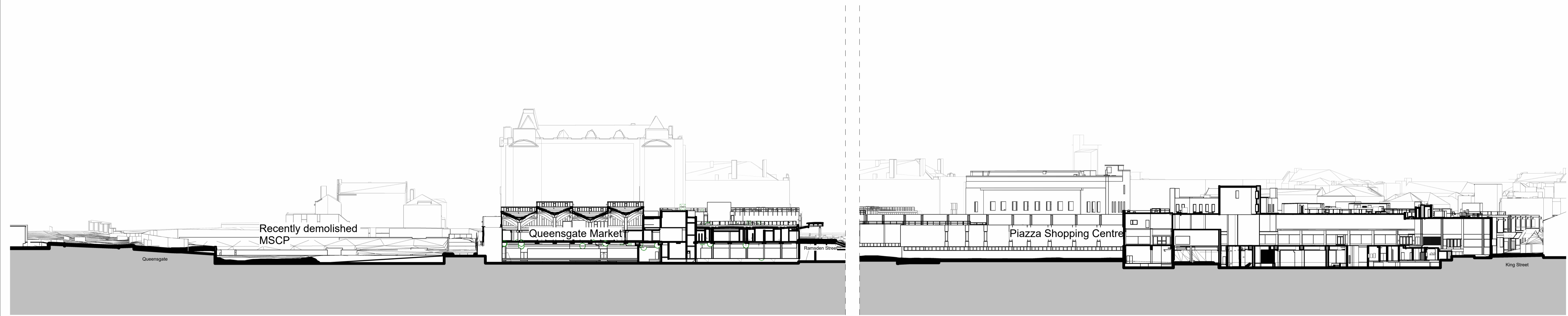
2 Section 2 - South North through the Existing Queensgate Market looking west 1 : 500
