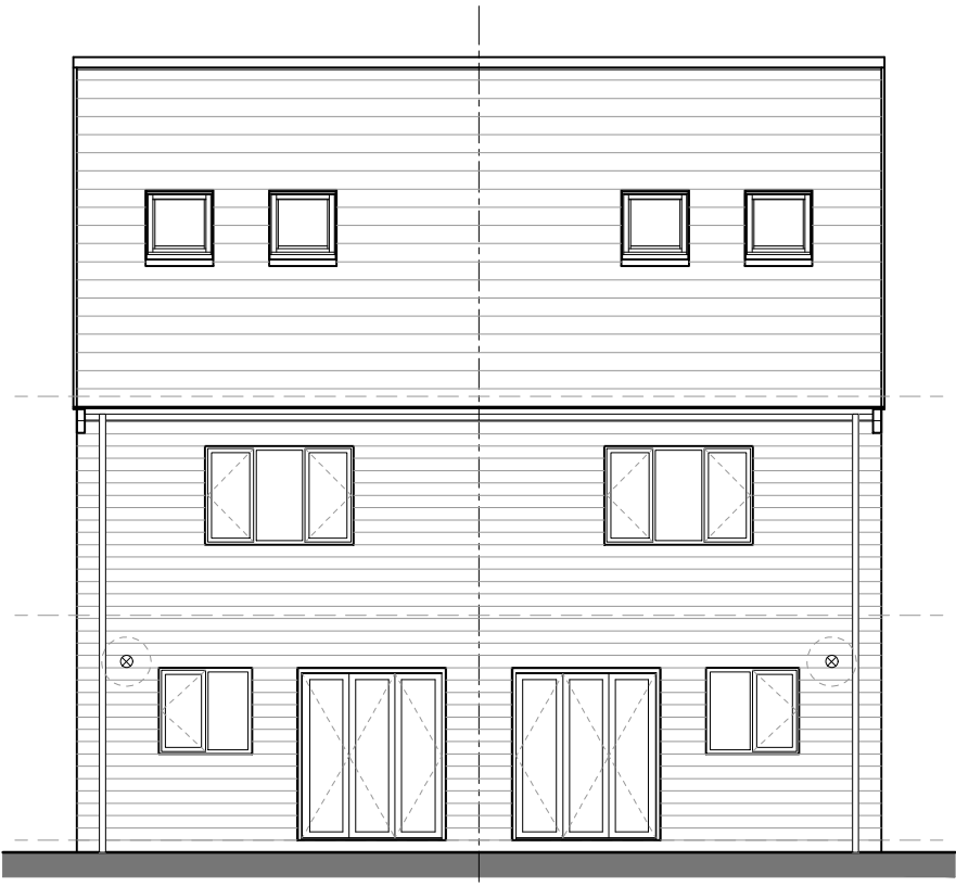
Rear Elevation
