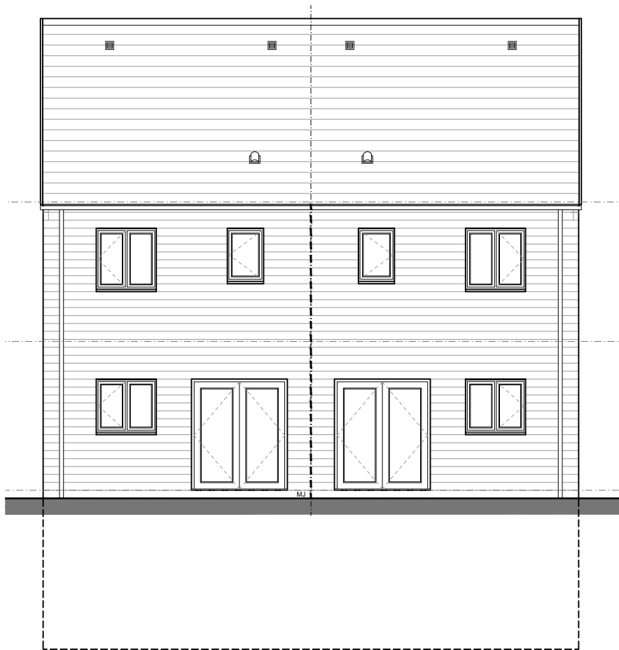
Rear Elevation
