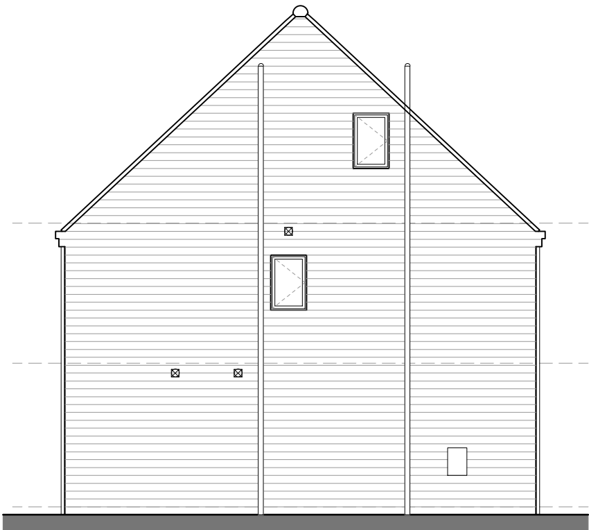
LH Gable Elevation
