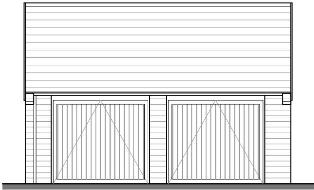
FRONT ELEVATION
