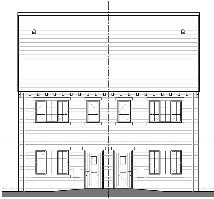
Front Elevation
