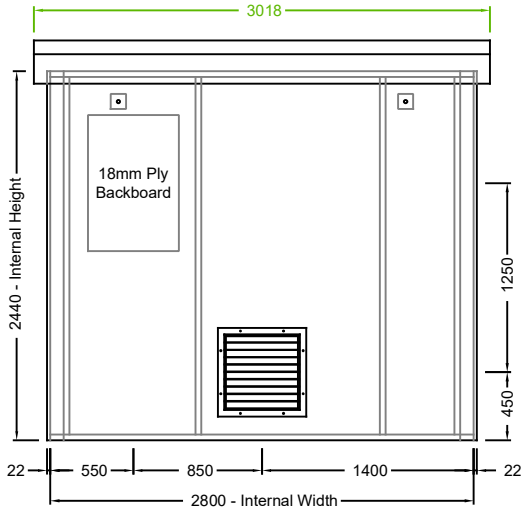
RH SIDE ELEVATION
