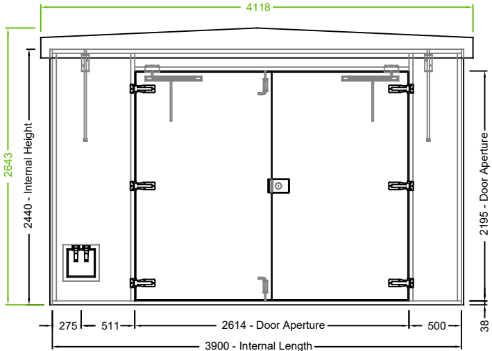
FRONT ELEVATION
