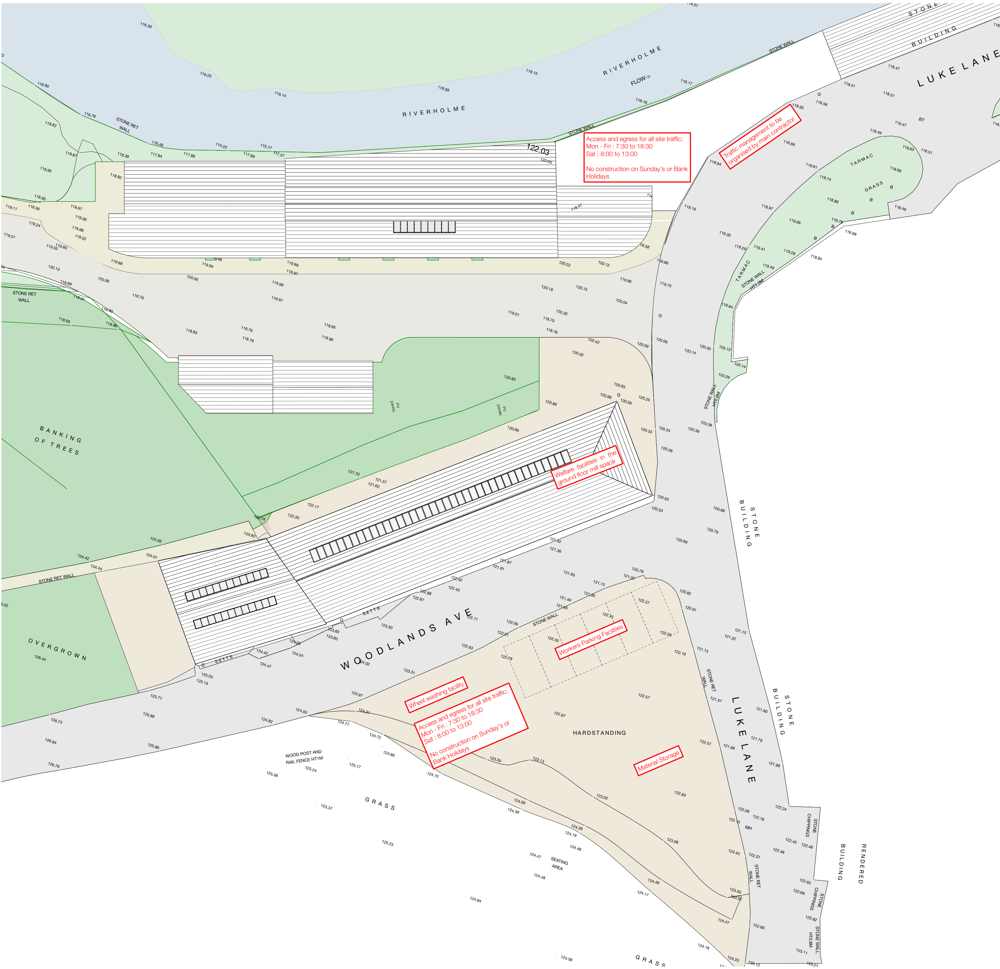
Construction Management Plan 1:200
