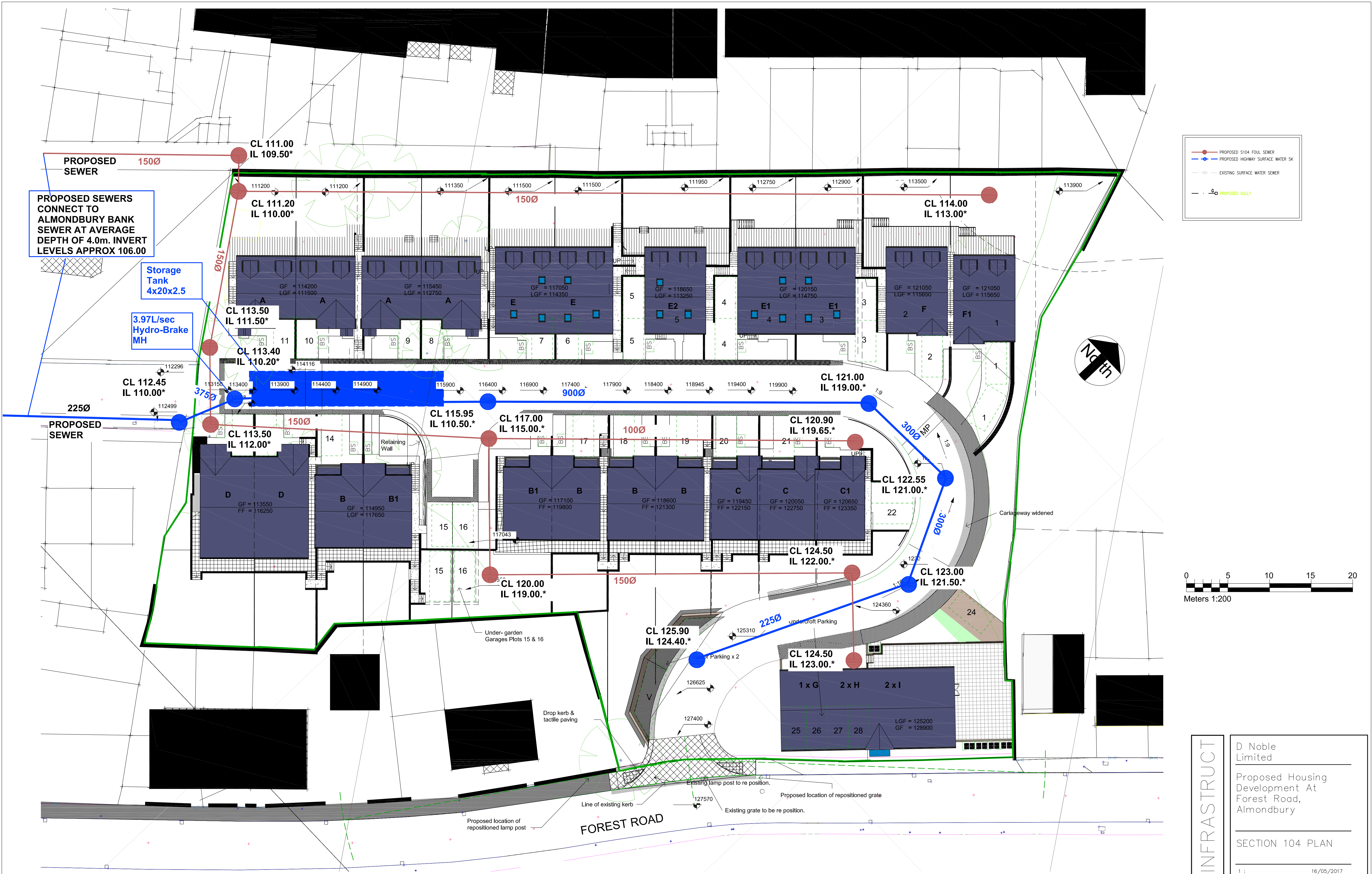
1 Proposed Housing Layout. Existing Topo Overlay 1 : 200
