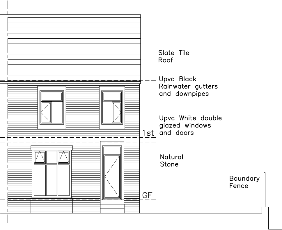
1:100 Scale Front Elevation as Existing
