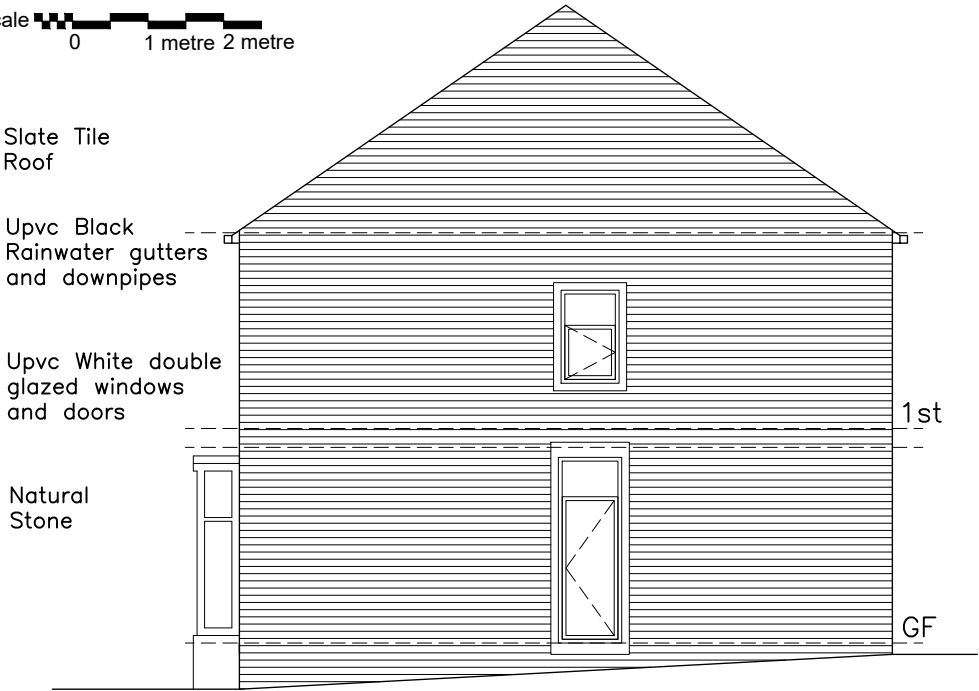
1:100 Scale Side Elevation as Existing
