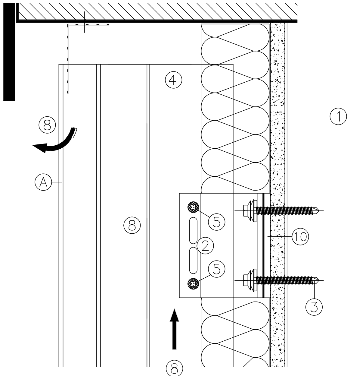
VERTICAL SECTION - TOP OF CLADDING
