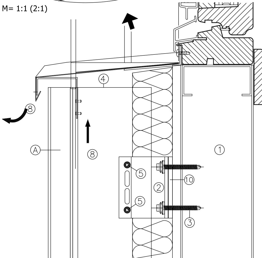
VERTICAL SECTION - WINDOW SILL DETAIL
