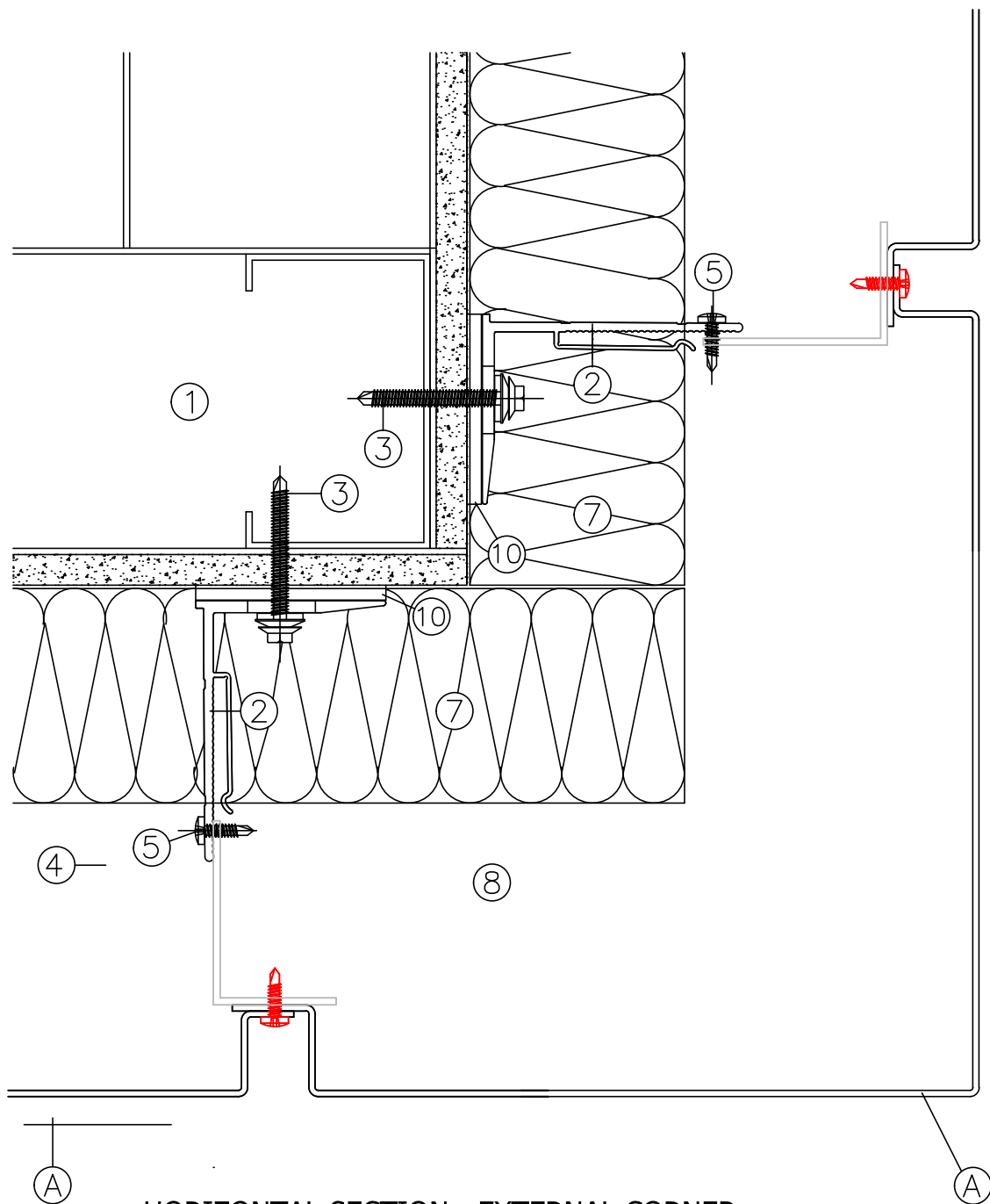
HORIZONTAL SECTION - EXTERNAL CORNER
