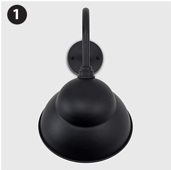
External Swan Neck Lights to shine on vinyl advertisement on roof surface. 60 watts, 1500 lumens, 3000k, IP67 rated.
