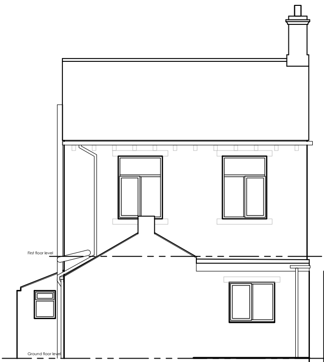
VIEW C - Existing Rear Elevation
