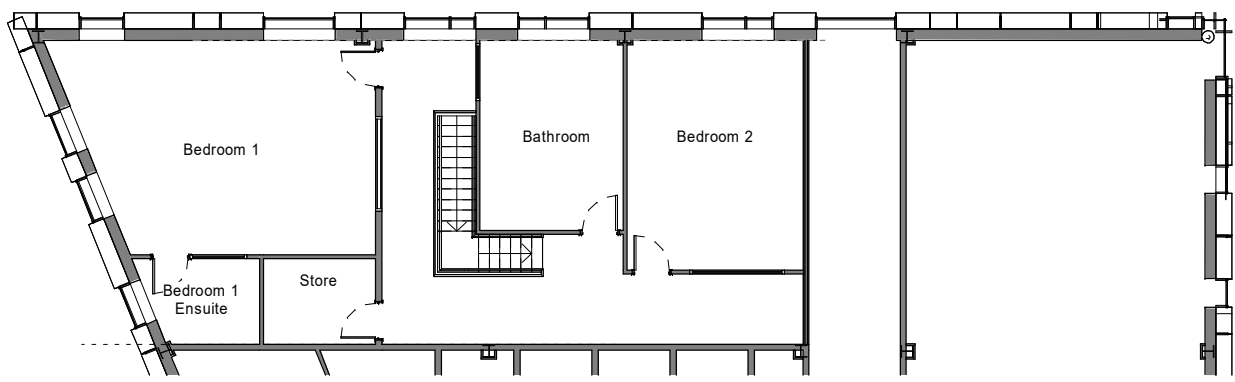
2 LEVEL 0.5 - Mezzanine 1 : 200
